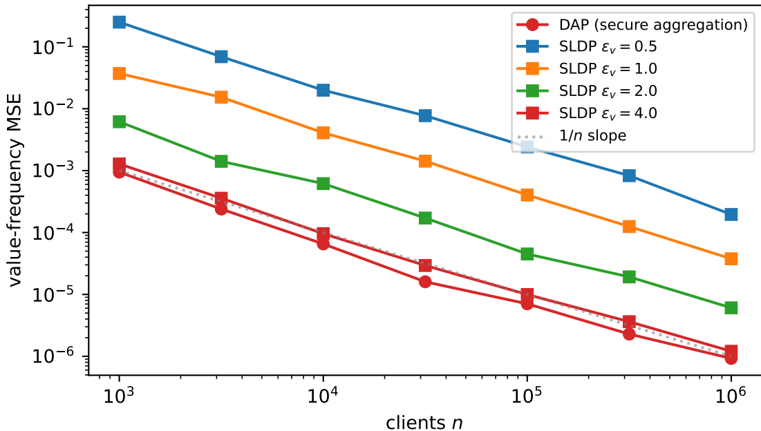
DAP vs SLDP value accuracy (K=10 categories)
