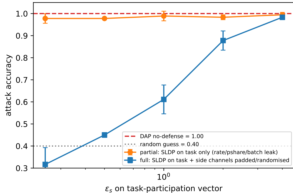
SLDP under non-collusion: partial vs full defense
