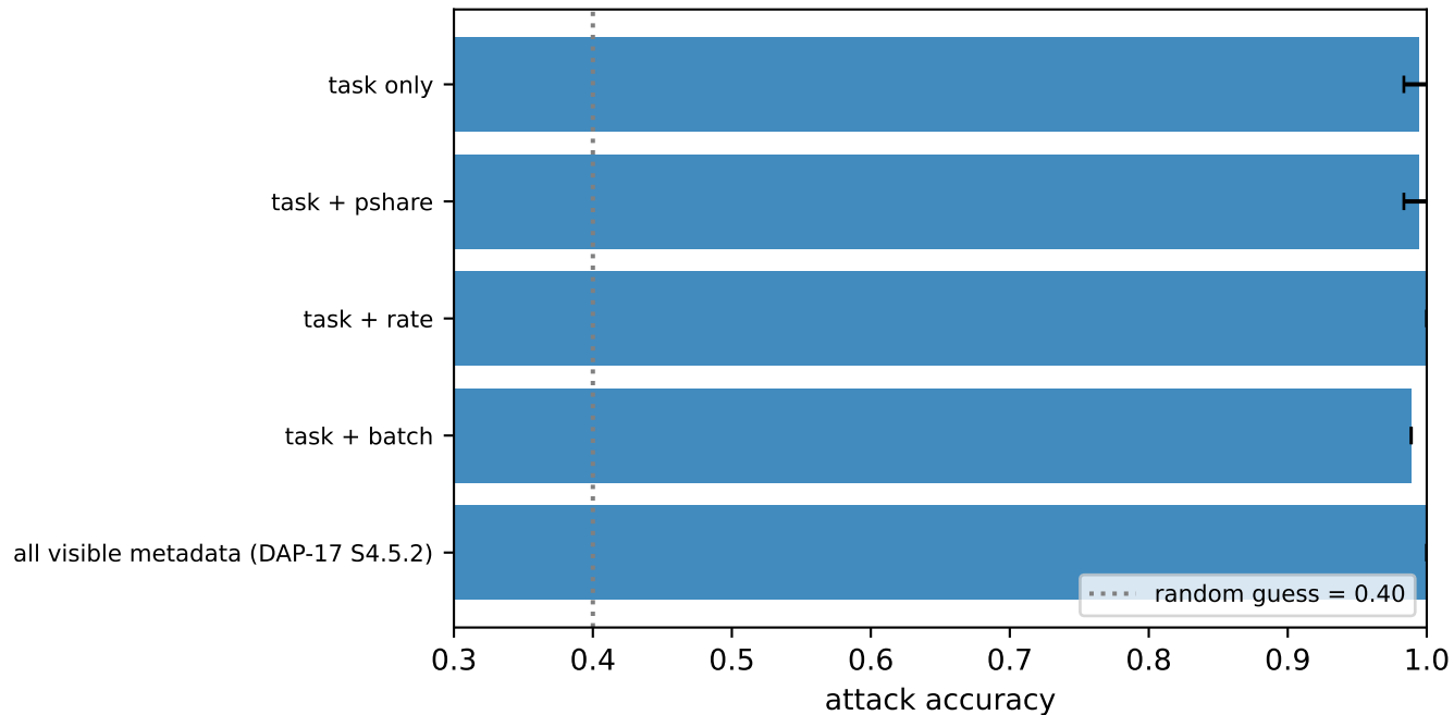
Non-collusion leak by metadata channel
