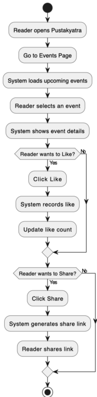
Activity Diagram 2 - Reader View/Like/Share Events (EMS) - Pustakyatra
