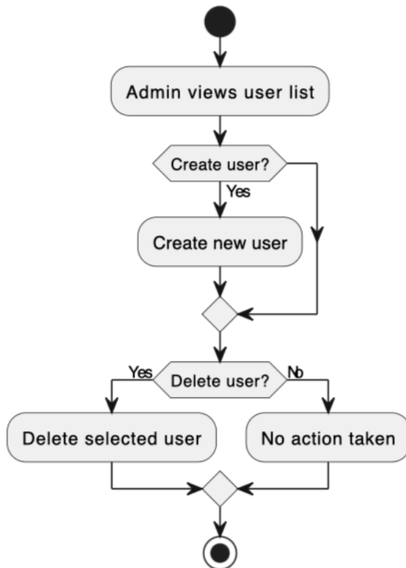
Figure 8: Activity Diagram 3 for UMS
