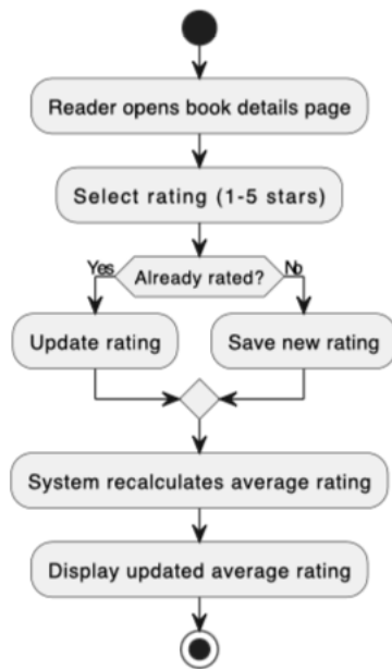
Activity Diagram 2 - Rating Management (CMS) - Pustakyatra
