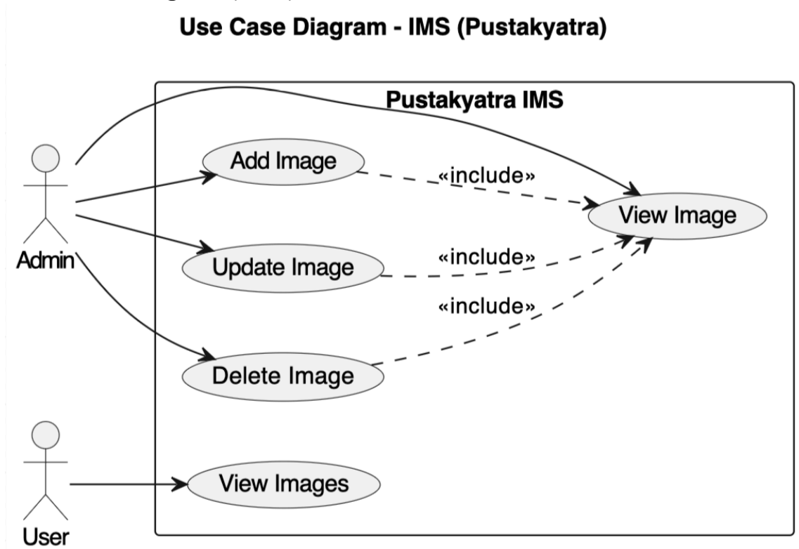
Figure 24: Use case Diagram of IMS
