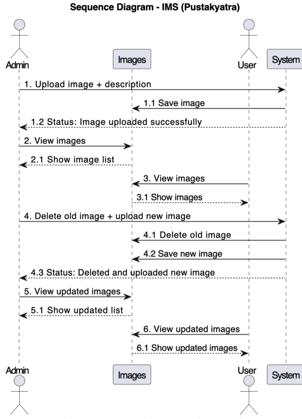
Figure 25: Sequence Diagram of IMS
