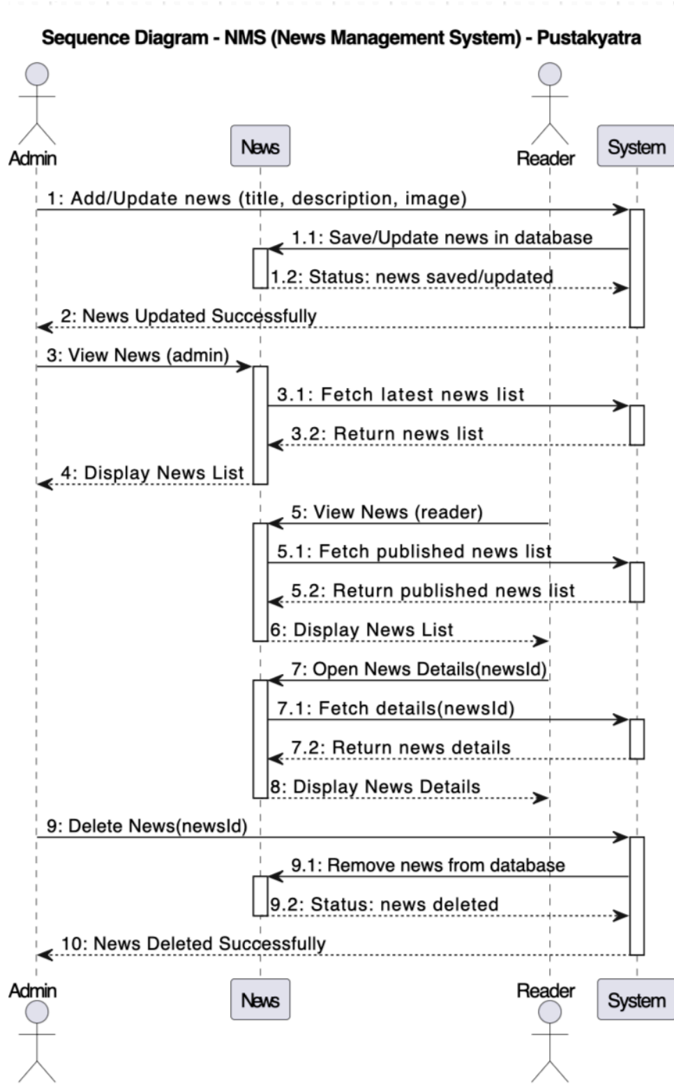
Figure 22: Sequence Diagram of NMS
