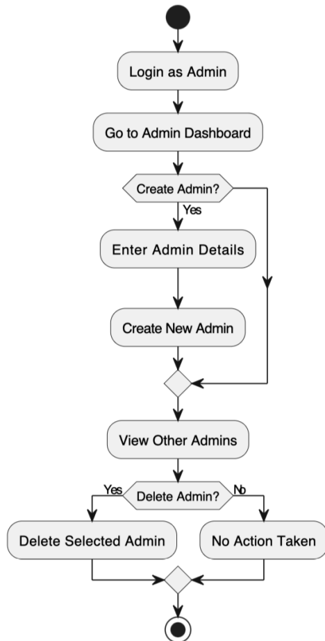
Activity Diagram - Create/Delete Admin (AMS)
