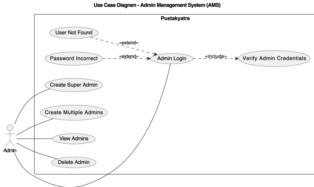
Figure 4: Use Case Diagram for Admin Management System (AMS)
