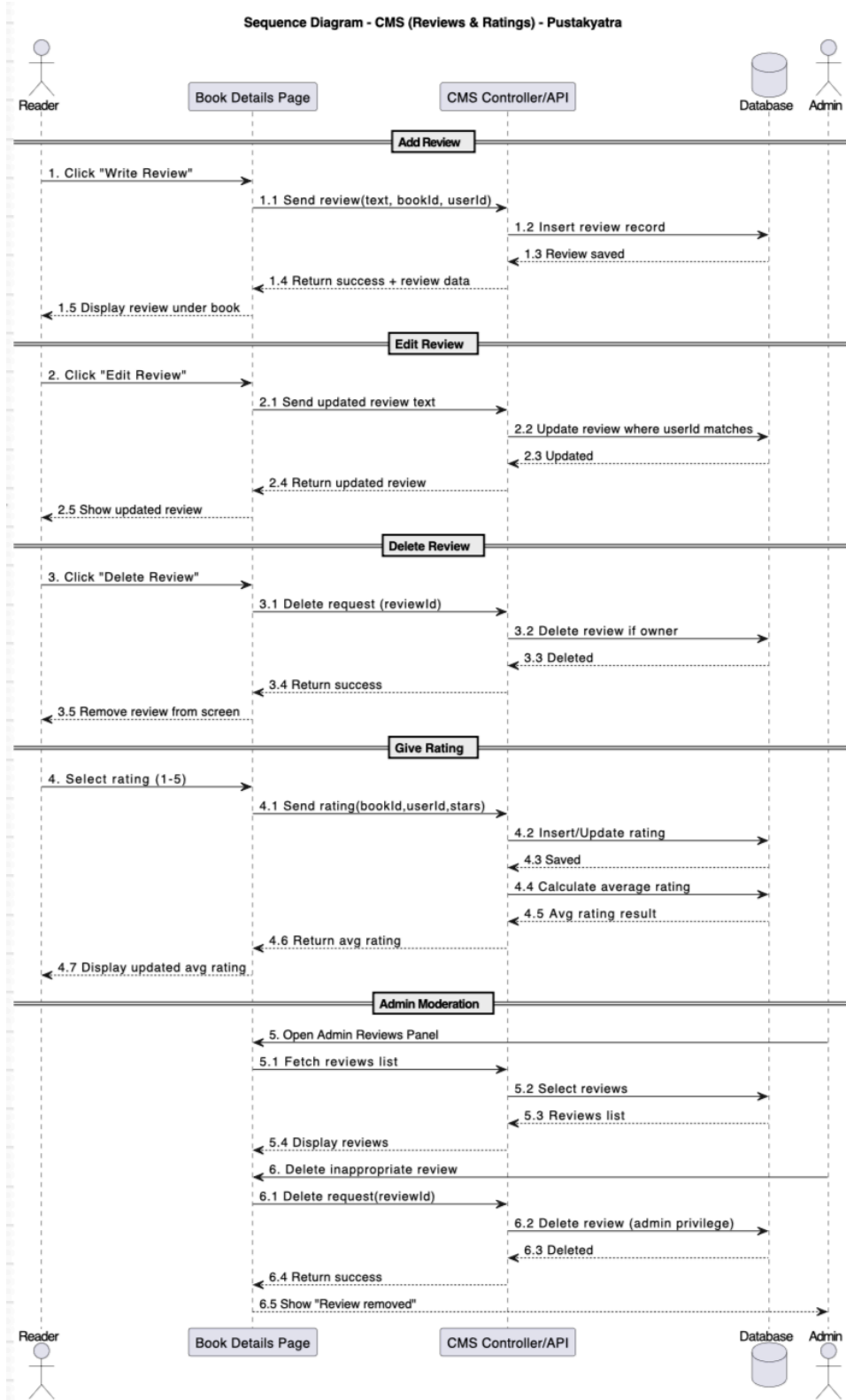
Figure 15: Sequence Diagram for CMS
