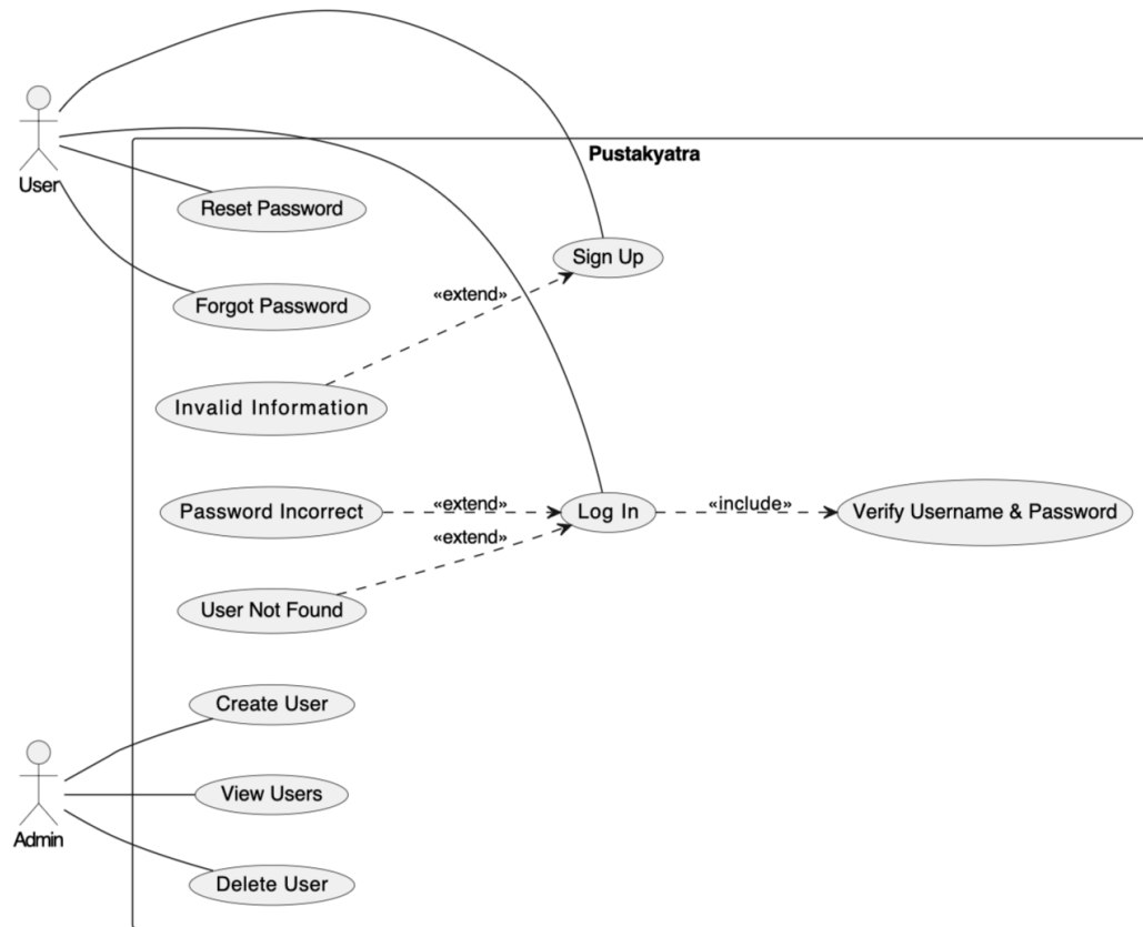
Figure 9: Use Case Diagram for UMS
