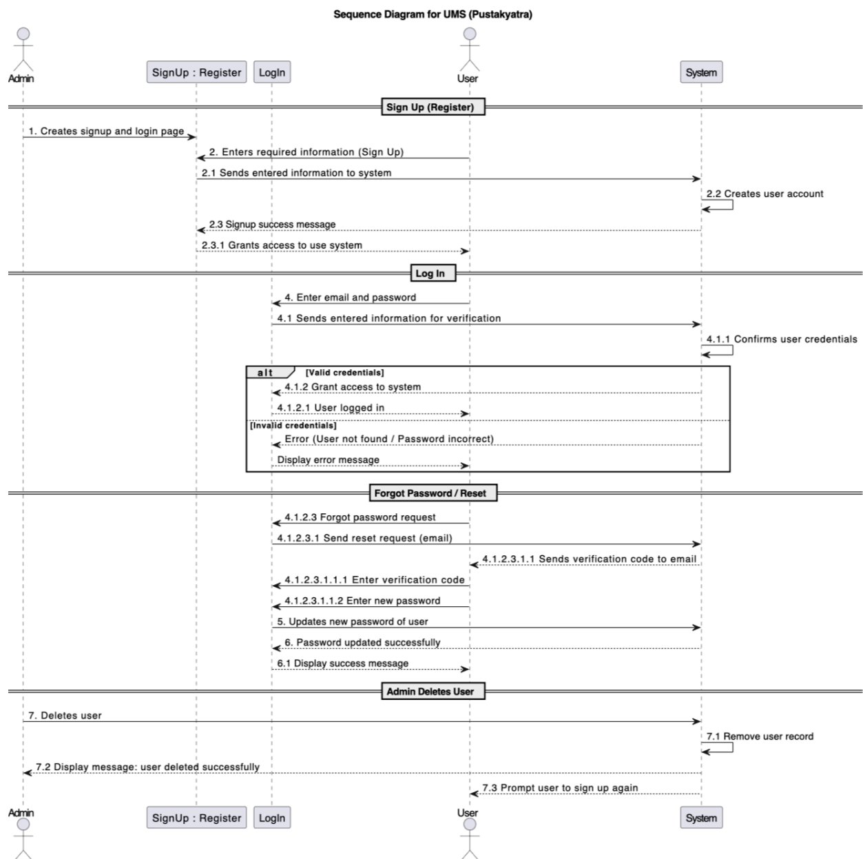
Figure 10: Sequence Diagram for UMS
