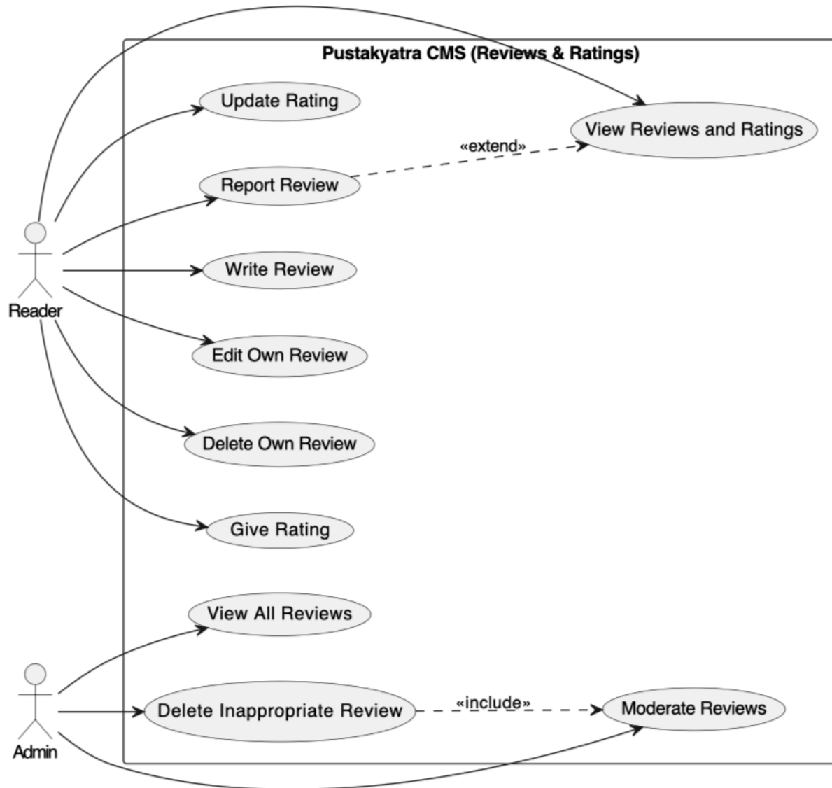
Figure 14: Use Case Diagram for CMS
