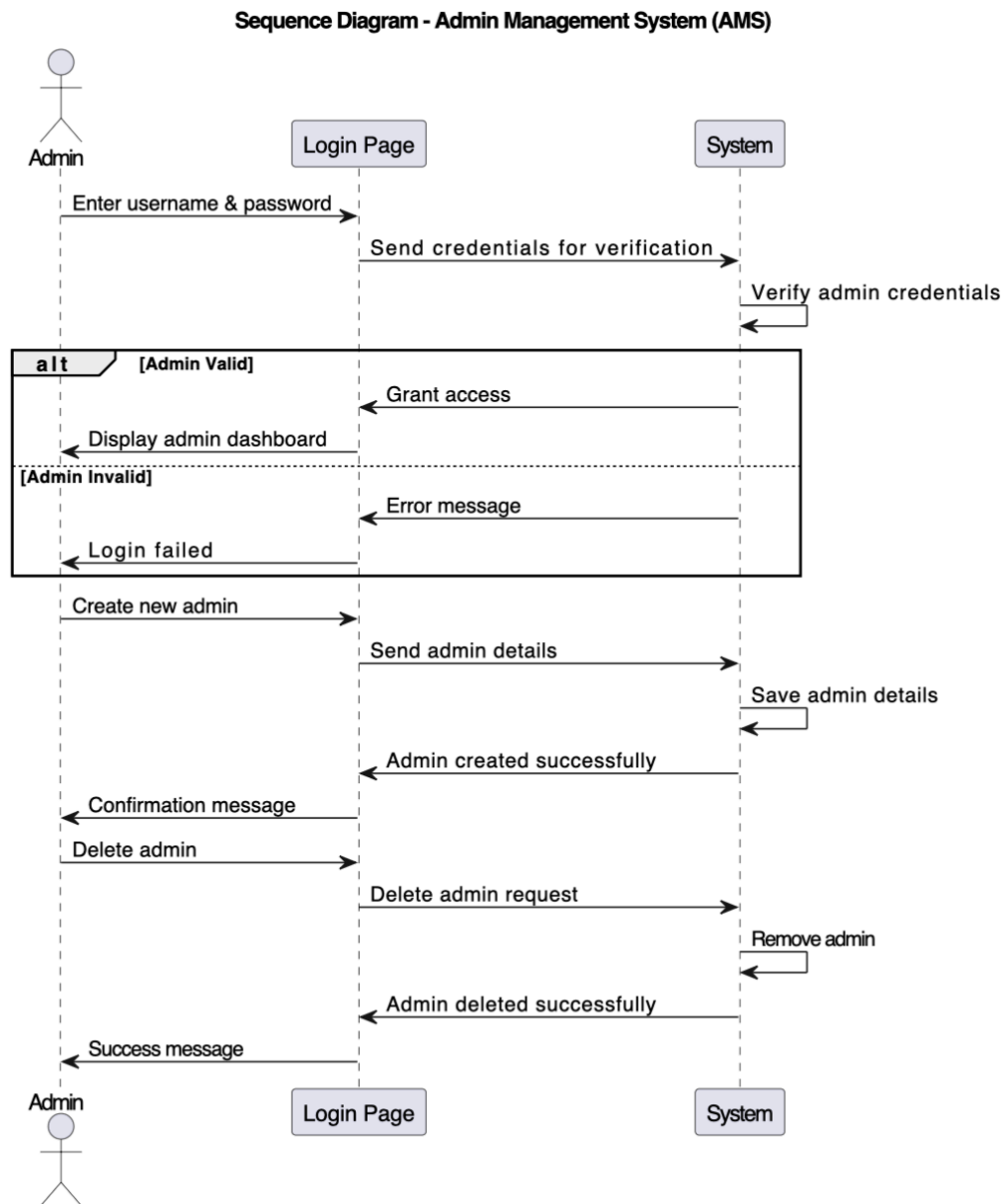
Figure 5: Sequence Diagram for Admin Management System (AMS)
