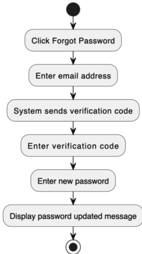
Figure 7: Activity Diagram 2 for UMS
