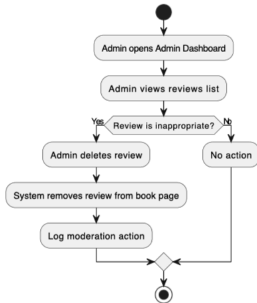
Figure 13: Activity Diagram 3 for CMS
