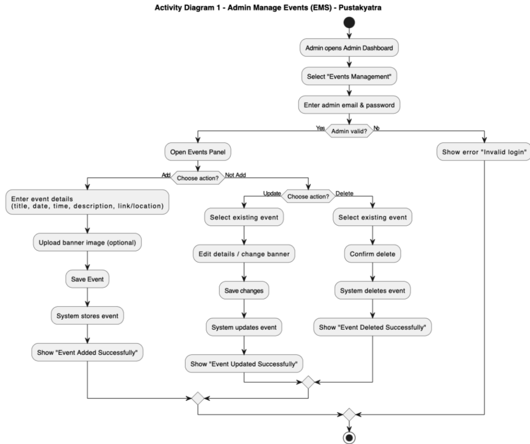
Figure 16: Activity Diagram (EMS)
