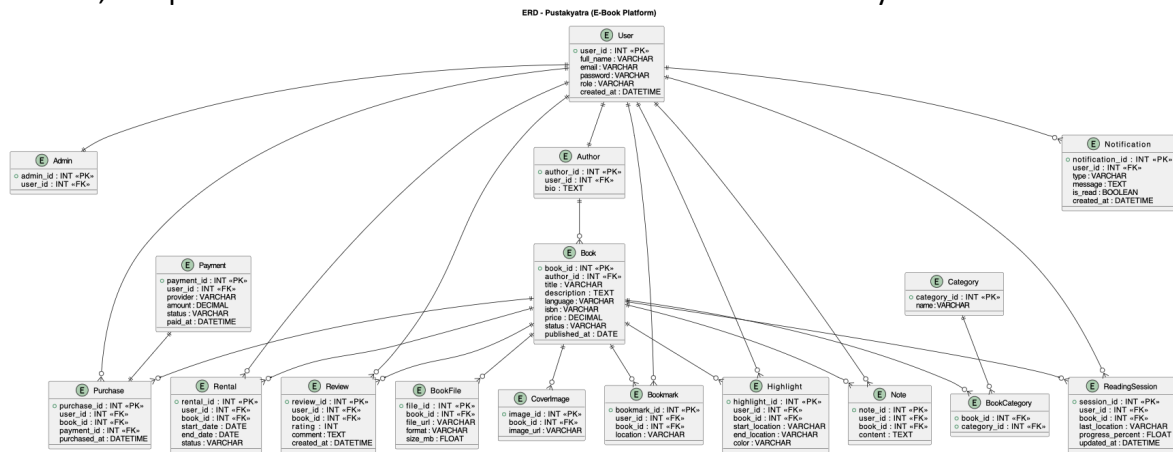
Figure 27: Entity-relationship Diagram of Pustakyatra
