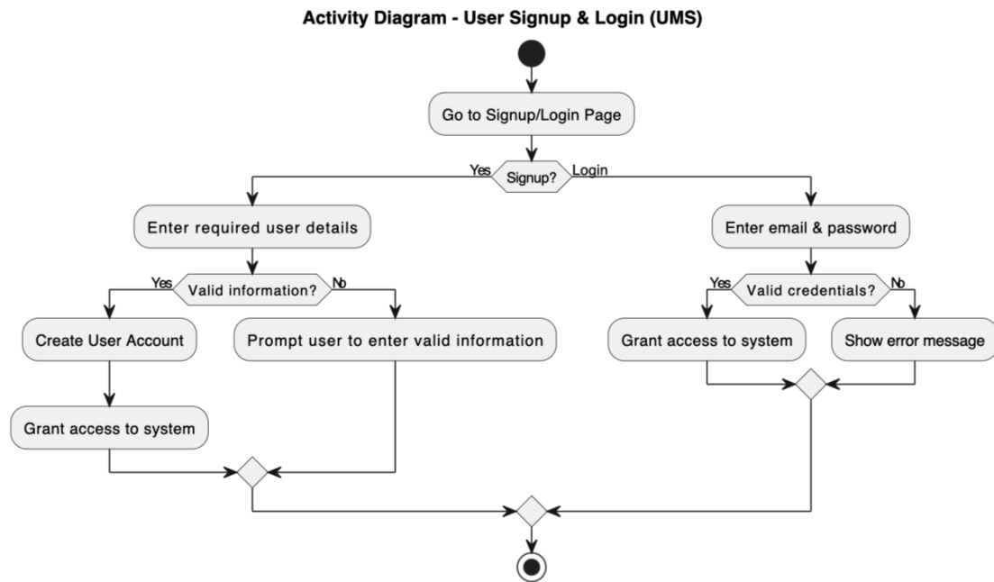
Figure 6: Activity Diagram 1 for UMS
