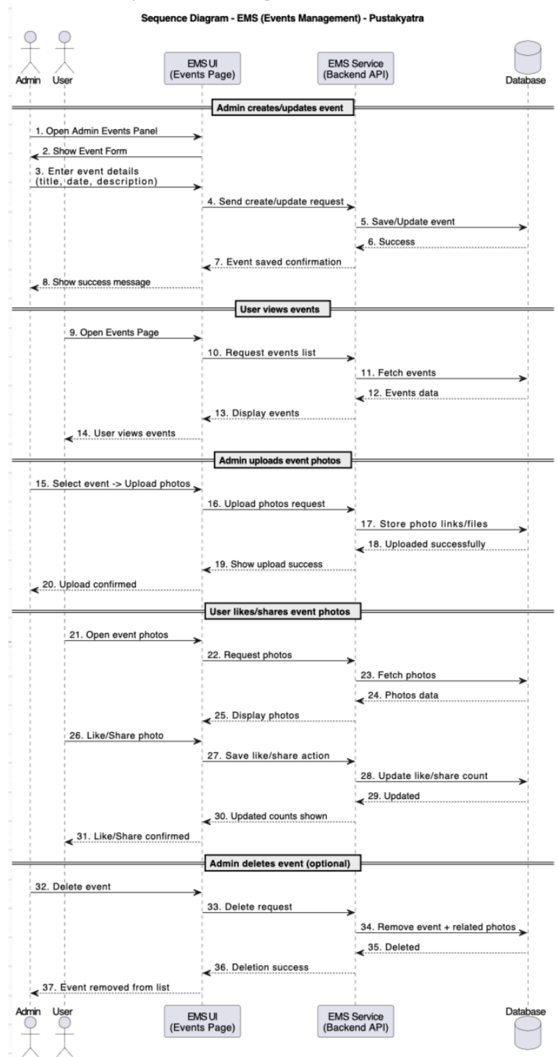
Figure 19: Sequence Diagram of EMS
