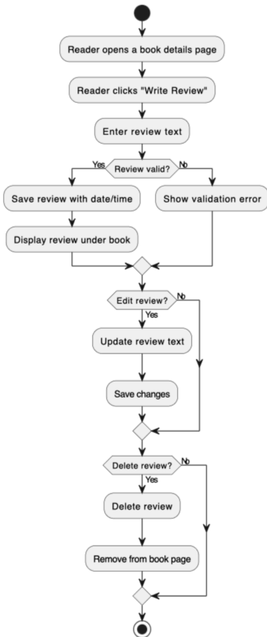
Activity Diagram 1 - Review Management (CMS) - Pustakyatra
