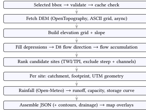
Fig. 2. The processing pipeline, from the selected area to the map overlays.
