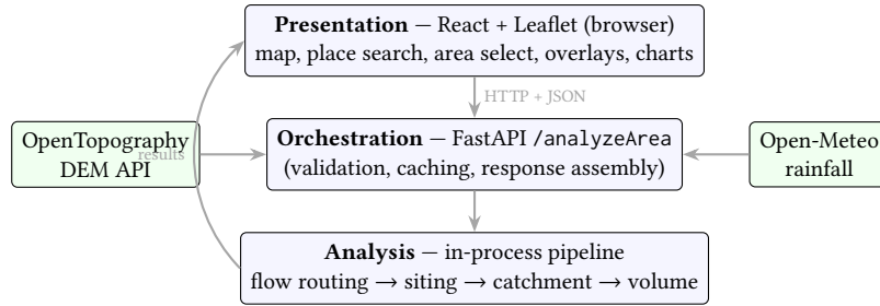
Fig. 1. High-level architecture. The single FastAPI process both serves the front-end and orchestrates the external data APIs and the analysis pipeline.
