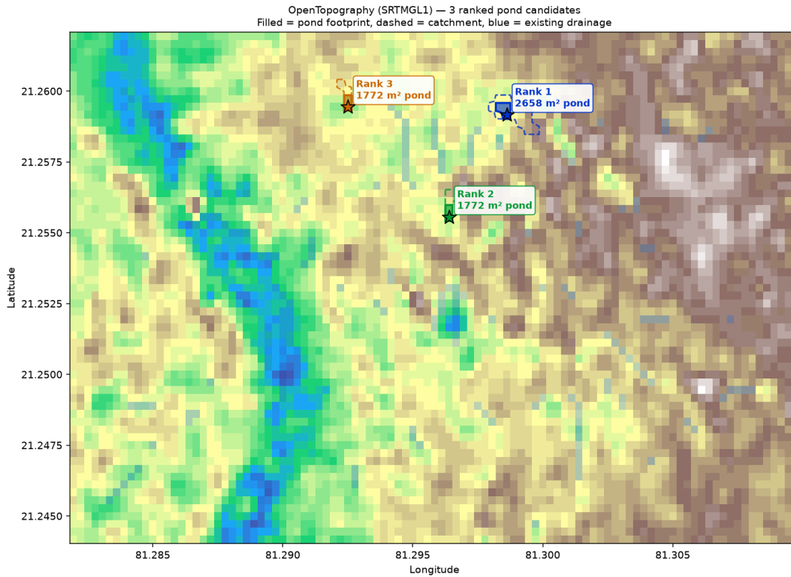
Fig. 3. Application results for the sample region: DEM terrain shading, the existing drainage network (blue), and three ranked pond sites (filled footprints) with their catchments (dashed), all kept off the watercourses.
