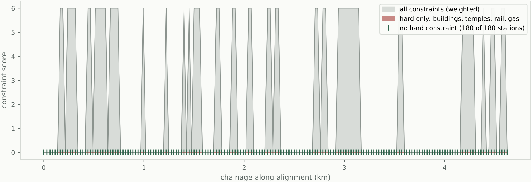
Constraint profile — what sits within a 8 m pier footprint, every 25 m
