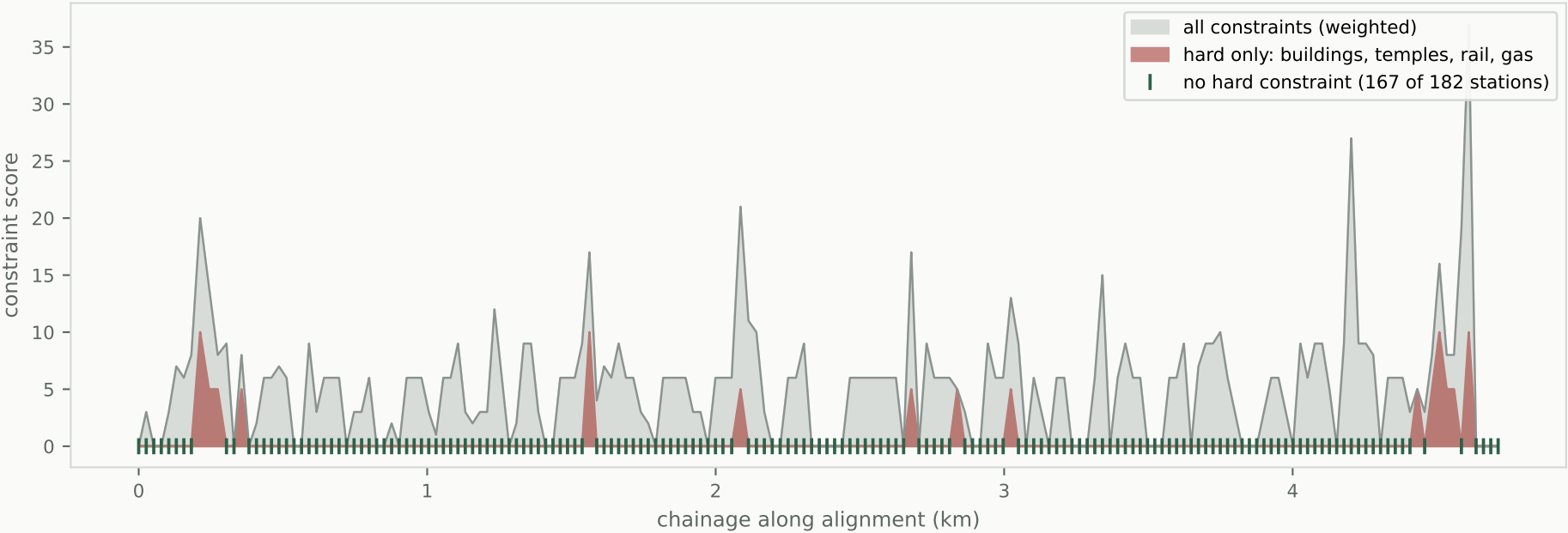
Constraint profile — what sits within a 8 m pier footprint, every 25 m
