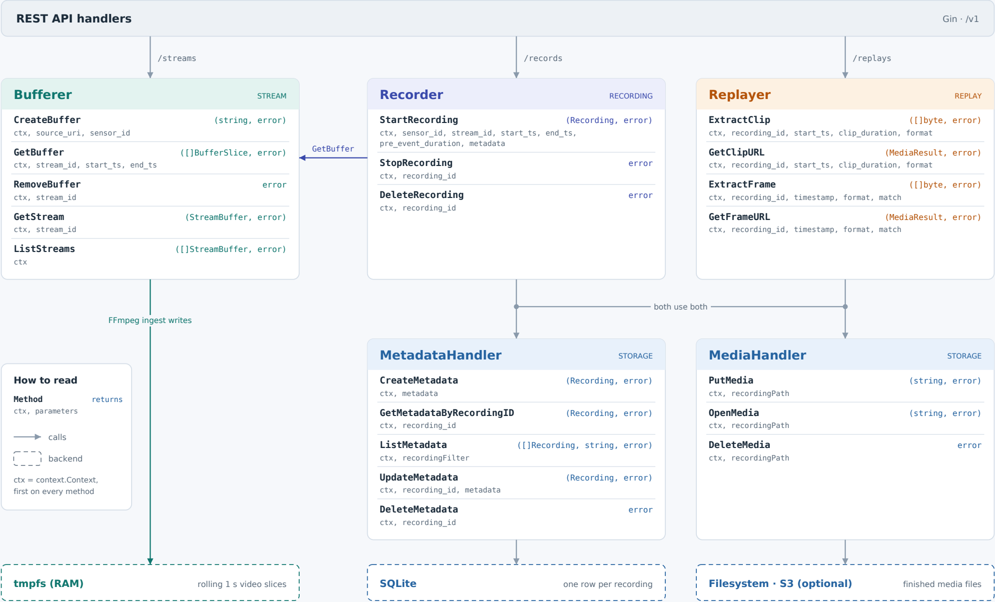
Figure 1 · API handlers call Bufferer, Recorder and Replayer; storage goes through MetadataHandler and MediaHandler.
