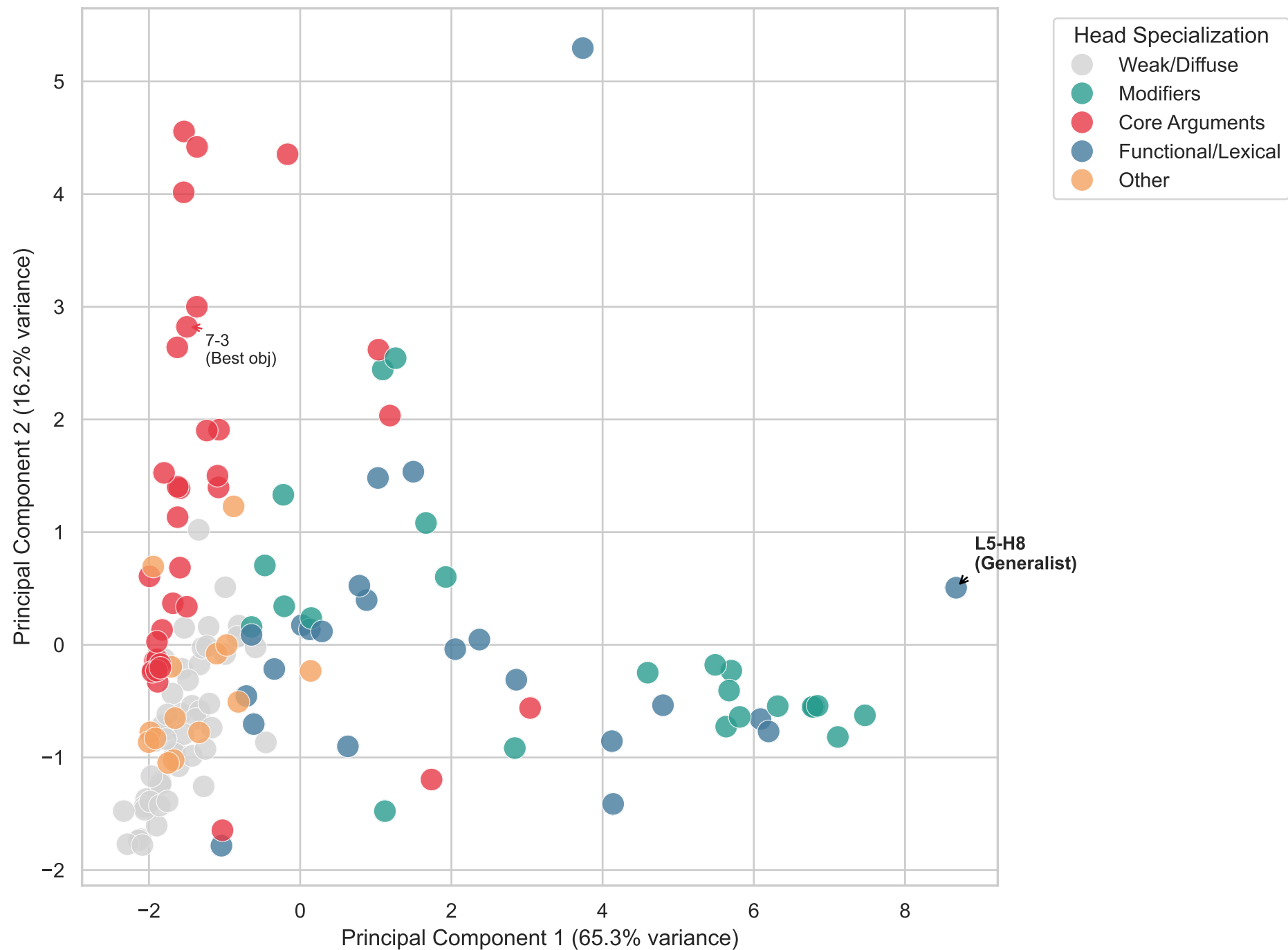
mBERT 'Brain Map': Attention Heads Clustered by Syntactic Specialization (PCA projection of 11-dimensional accuracy vectors)
