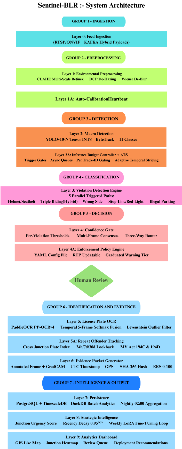
Figure 2: Sentinel-BLR Full System Architecture
