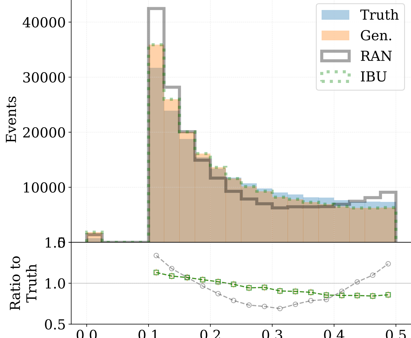
Groomed Jet Momentum Fraction (particle level)
