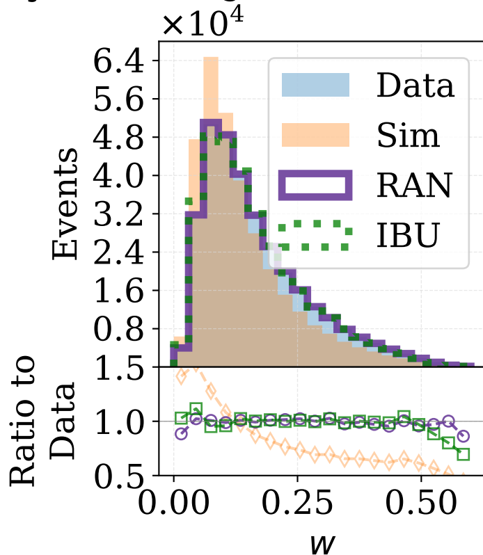
Jet Width
