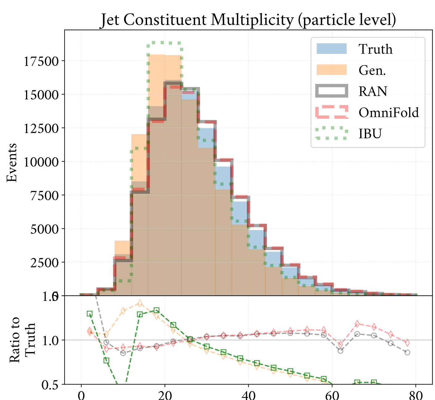
Jet Constituent Multiplicity (particle level)
