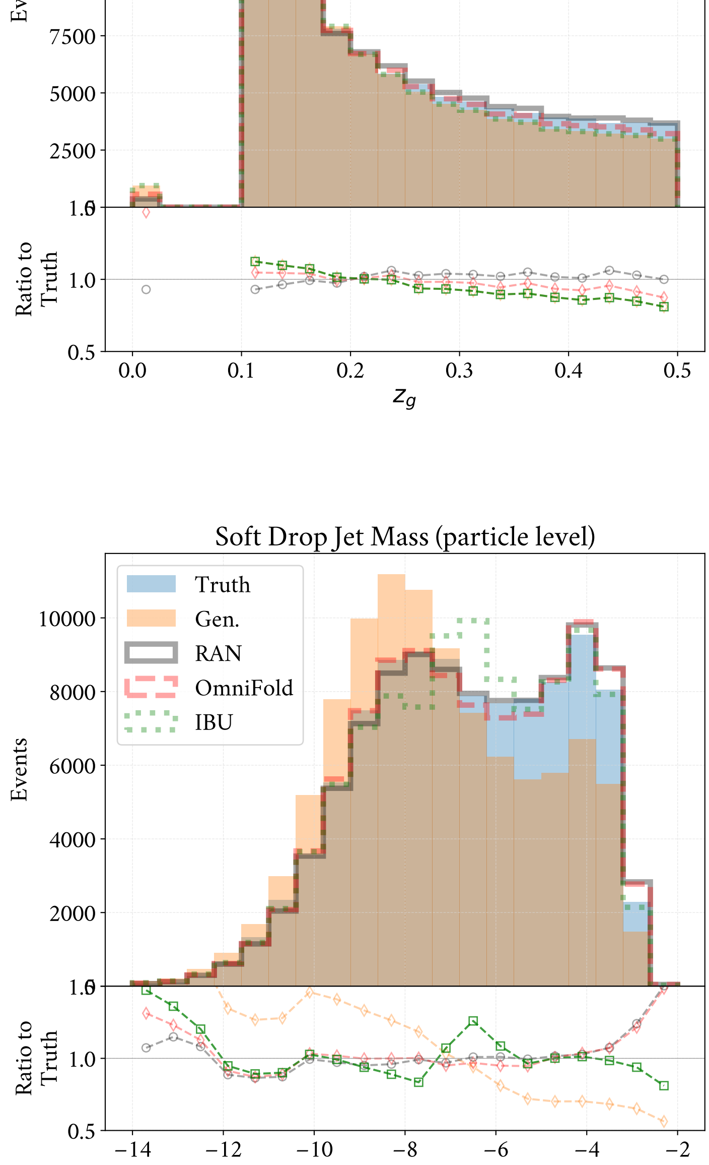
Soft Drop Jet Mass (particle level)
