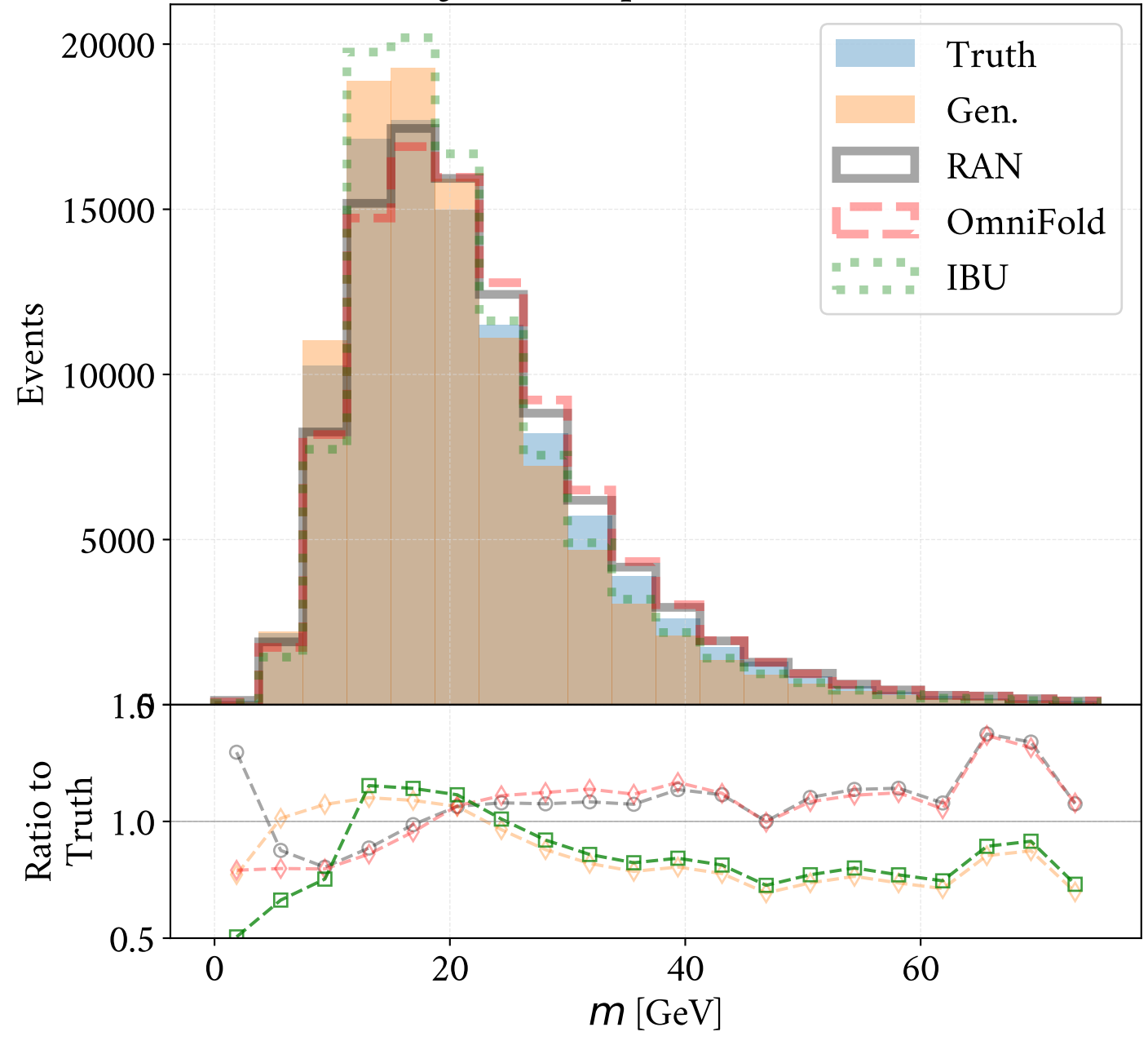
Jet Mass (particle level)
