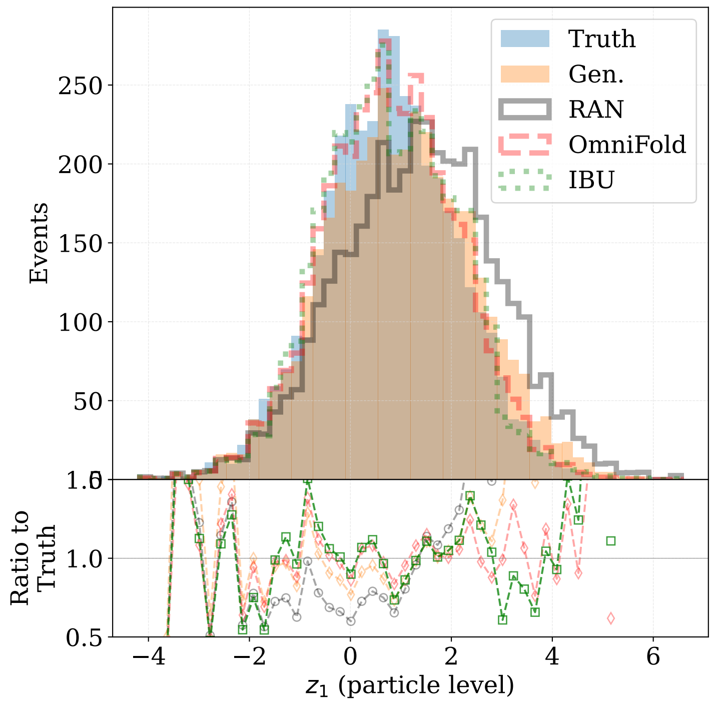
Particle Level — Dim 1
