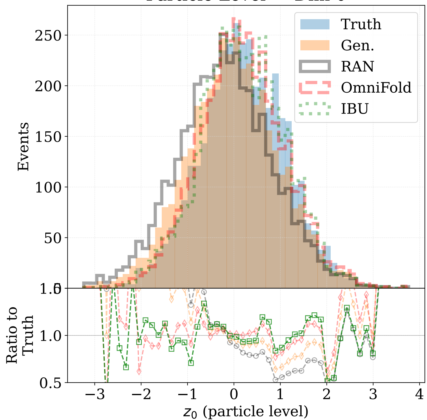
Particle Level — Dim 0
