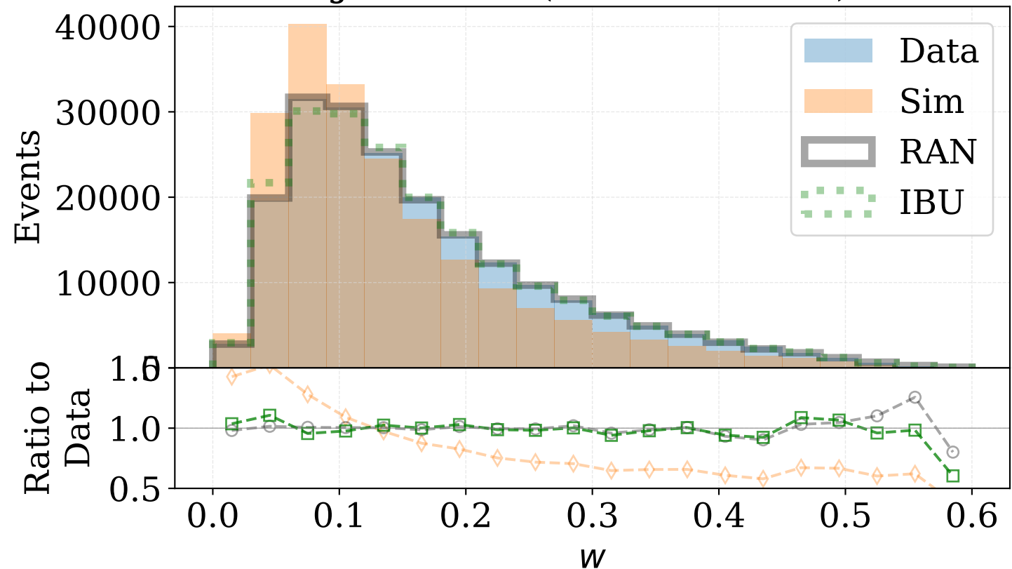
Jet Width (detector level)
