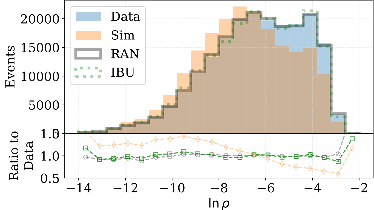
Soft Drop Jet Mass (detector level)
