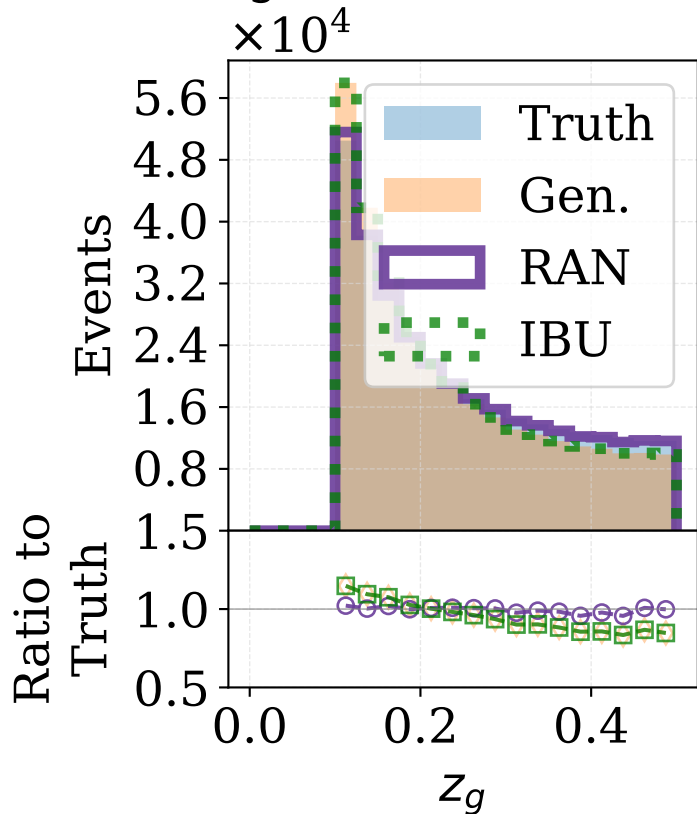
Groomed Jet Momentum Fraction
