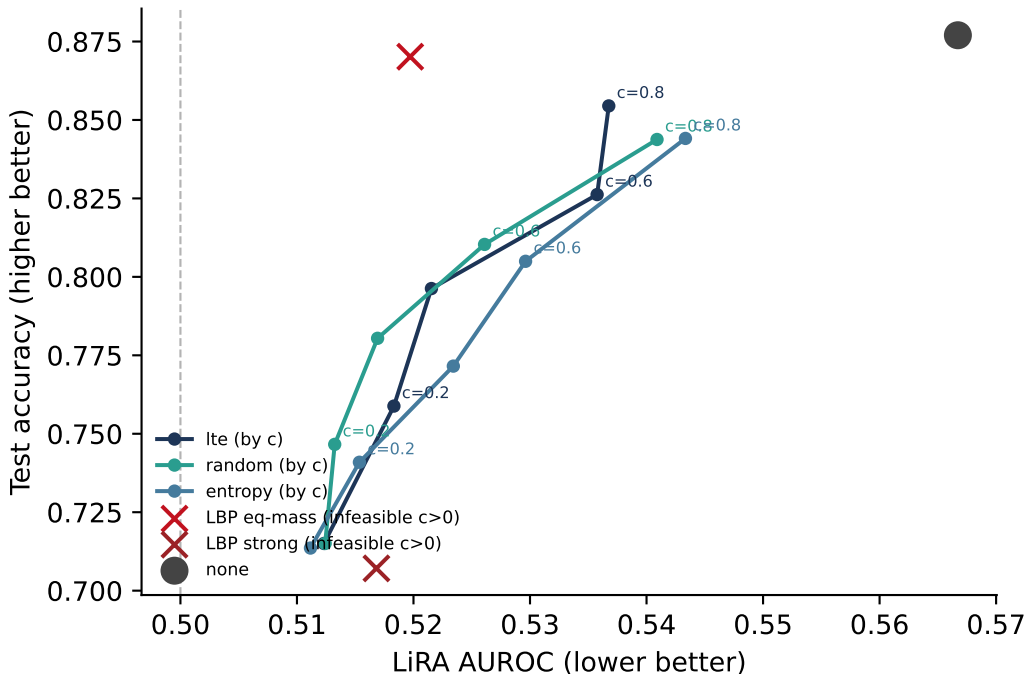
ExactFrac-constrained Acc-LiRA Pareto (Cora, 5 seeds)
