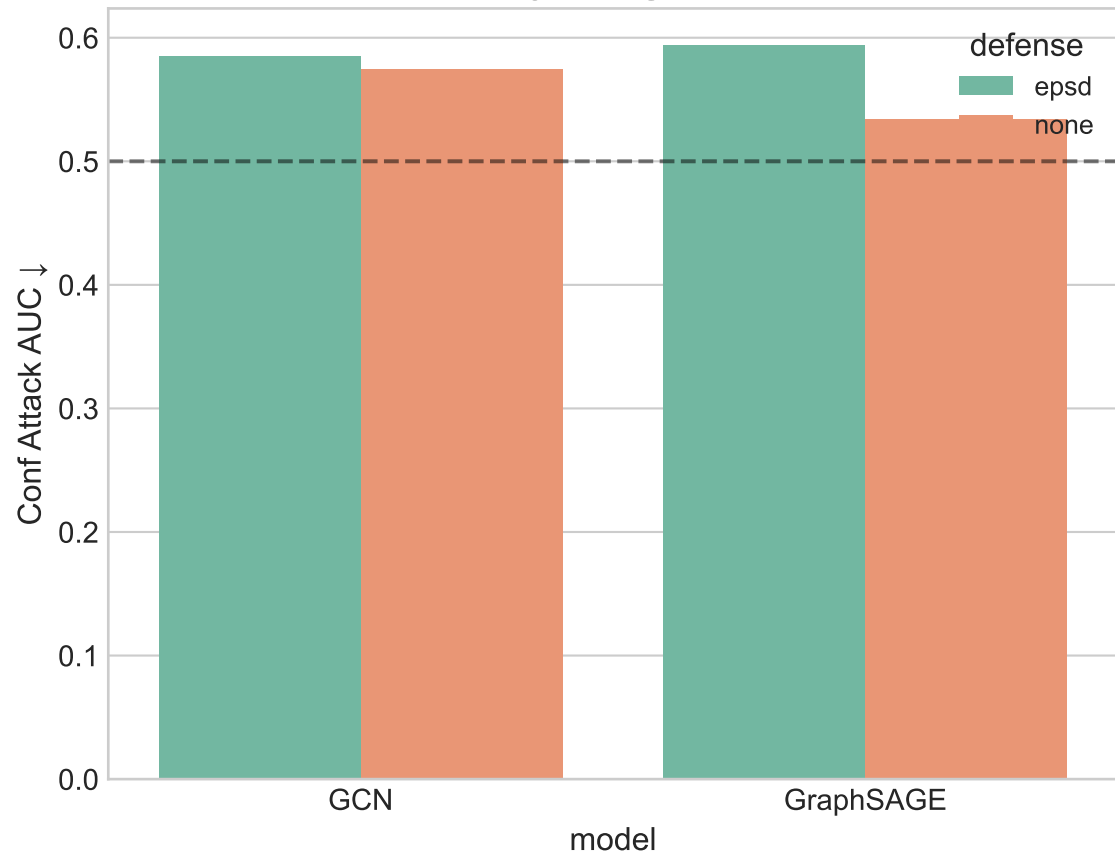
Privacy on ogbn-arxiv
