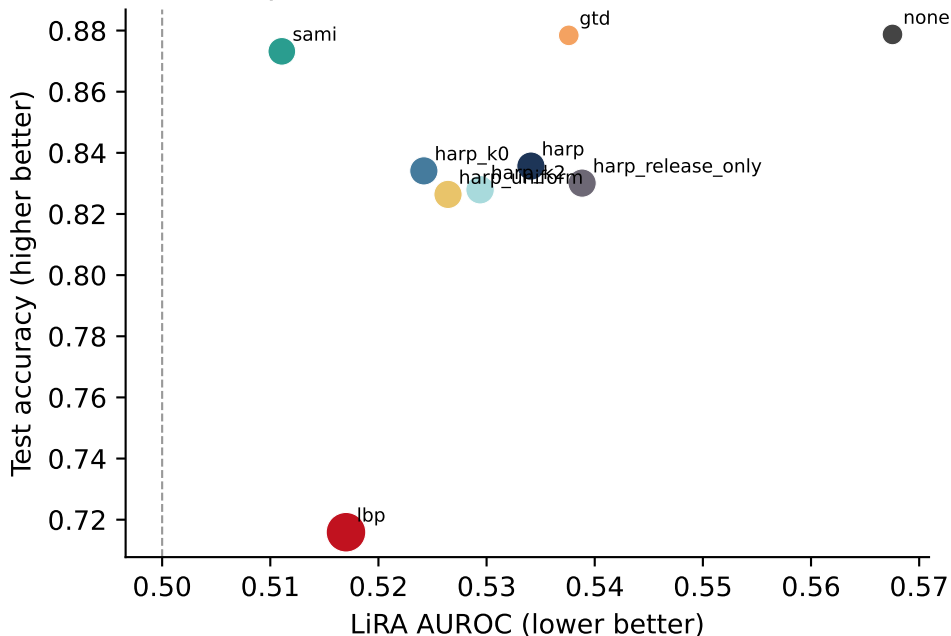
Cora GraphSAGE: Acc-LiRA (marker \propto noise mass)
