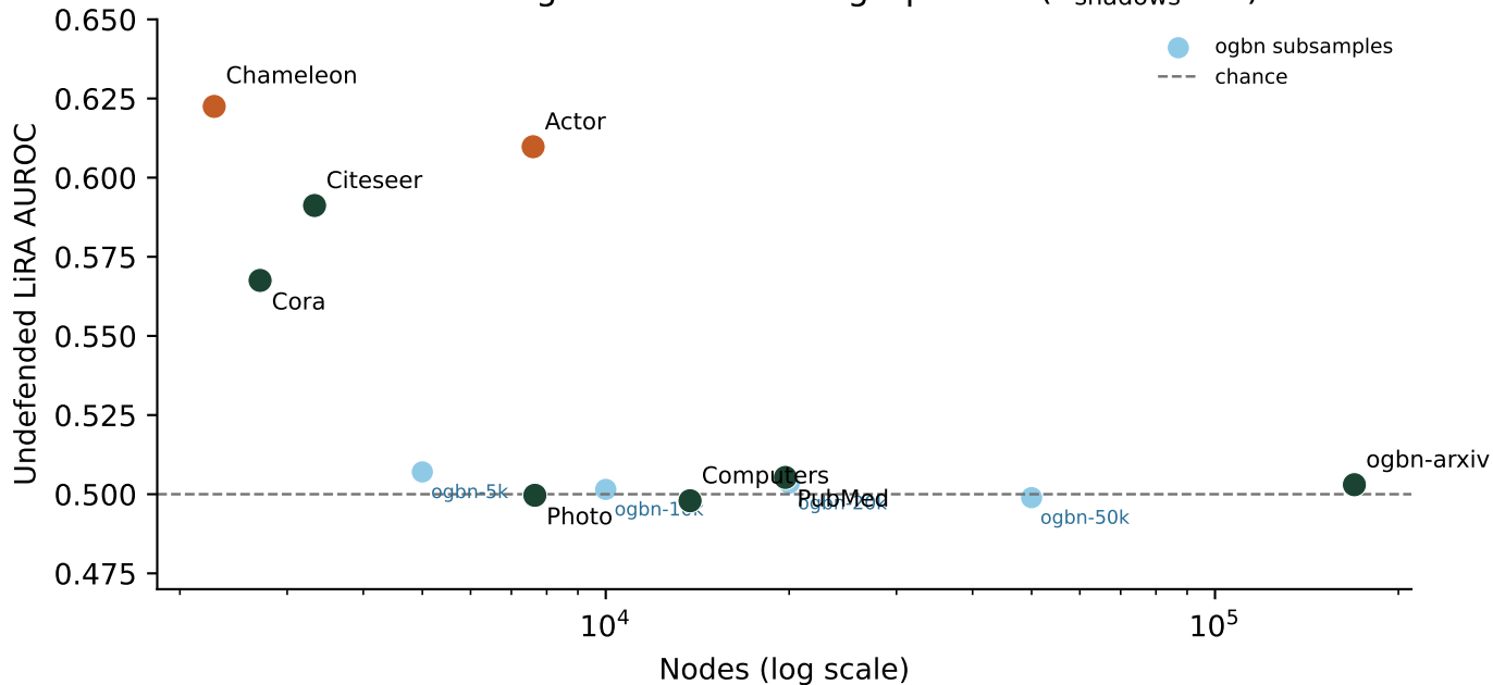
Matched-budget score LiRA vs graph size ( n_{\text{shadows}} = 4 )
