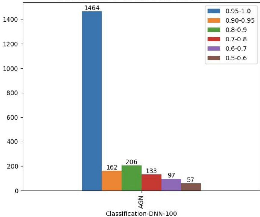
2119 unassociated sources AGN classification
