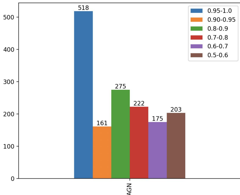
1554 unassociated sources AGN classification
