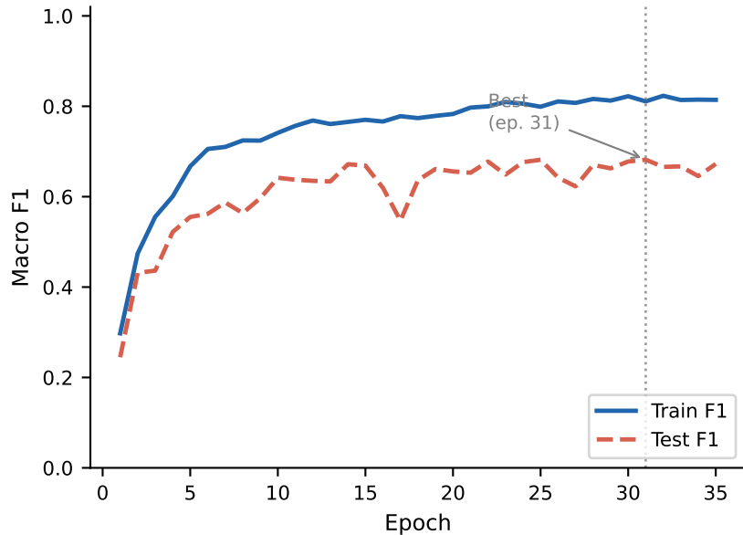
Pose-LSTM (Skeleton-Based)
