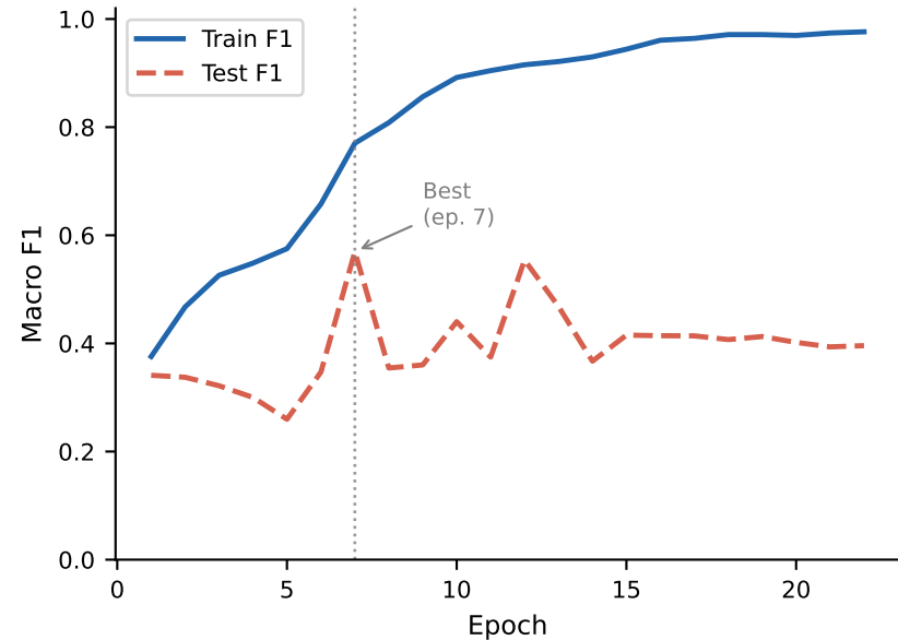
ResNet-18 (Transfer Learning)
