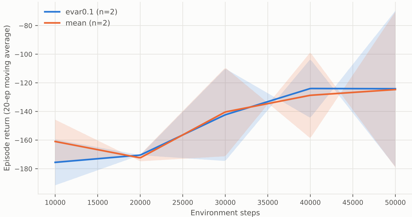
Learning curves - dsac-pendulum
