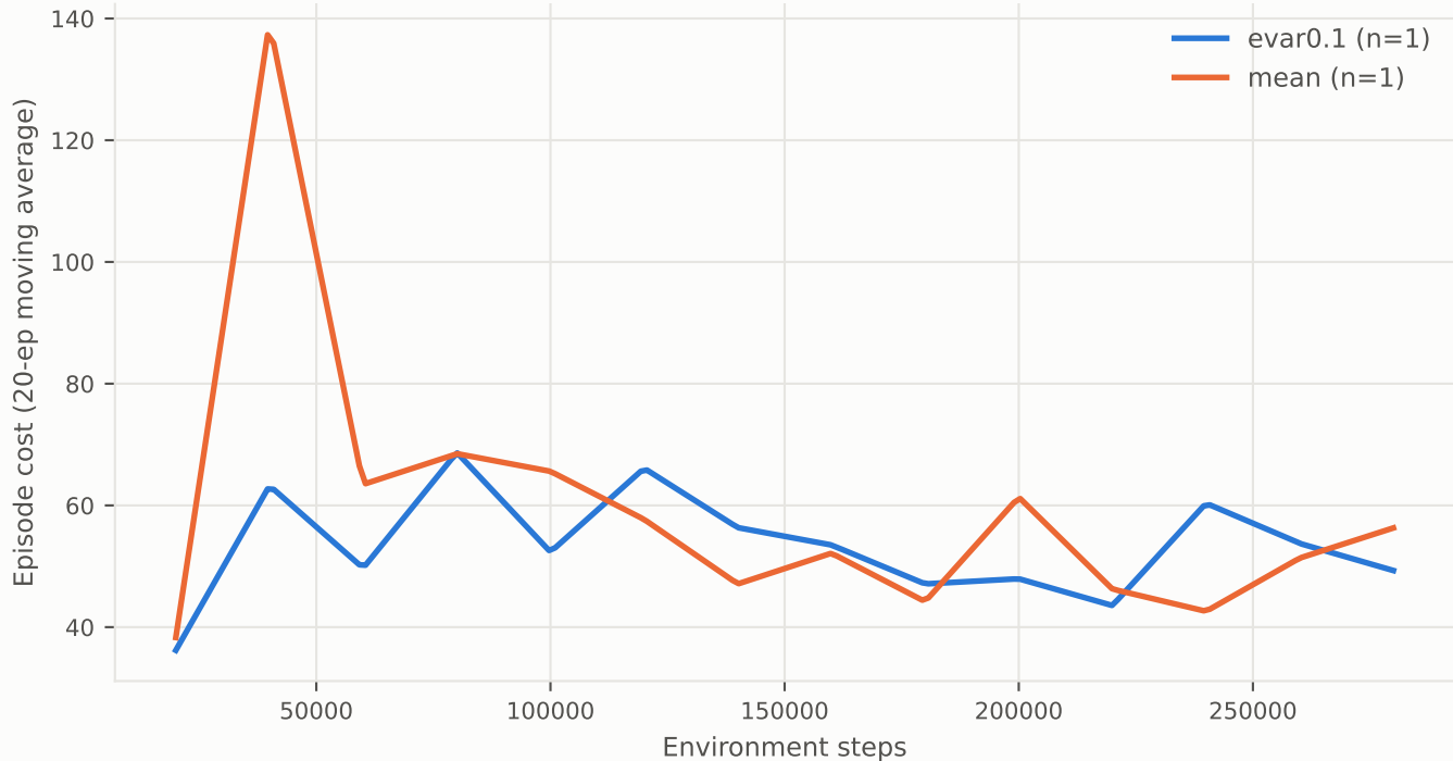
Safety cost incurred - dsac-safety-nav
