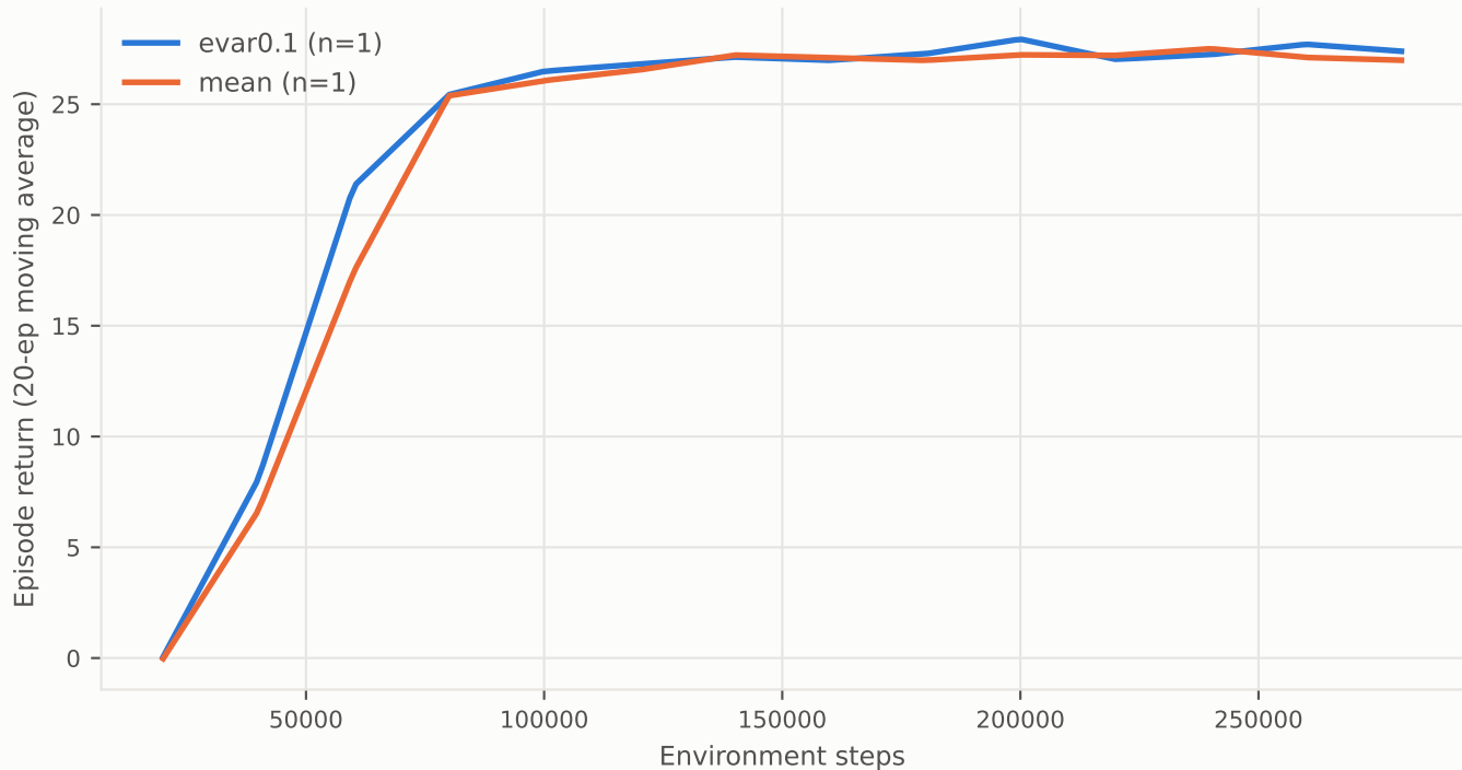
Learning curves - dsac-safety-nav
