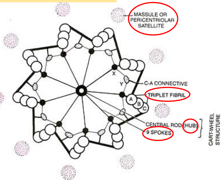
Fig: Ultrastructure of centriole as seen in T.S.
