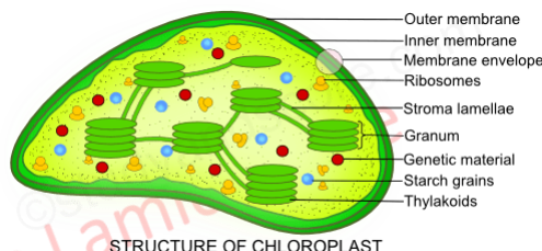
STRUCTURE OF CHLOROPLAST
