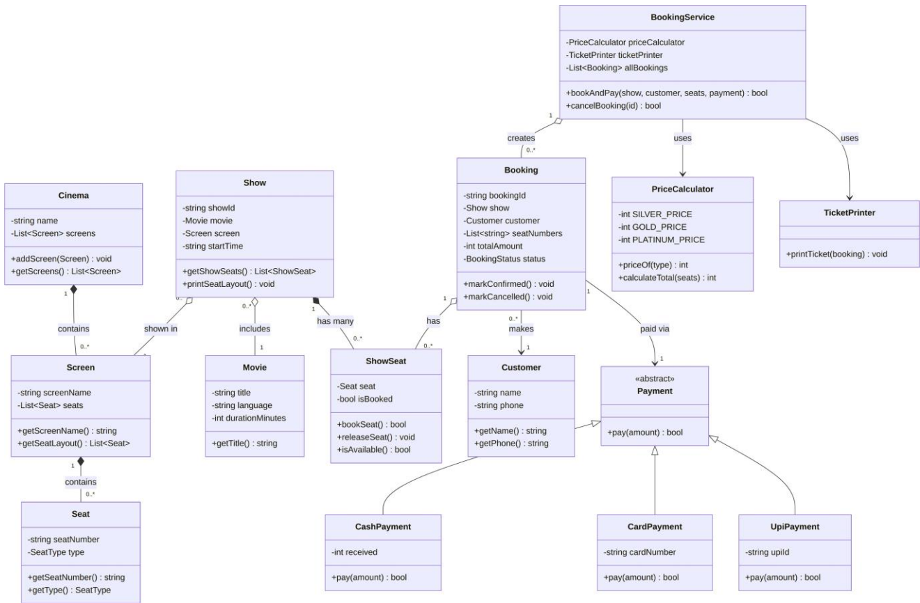
Movie Ticket Booking System — Class Diagram
