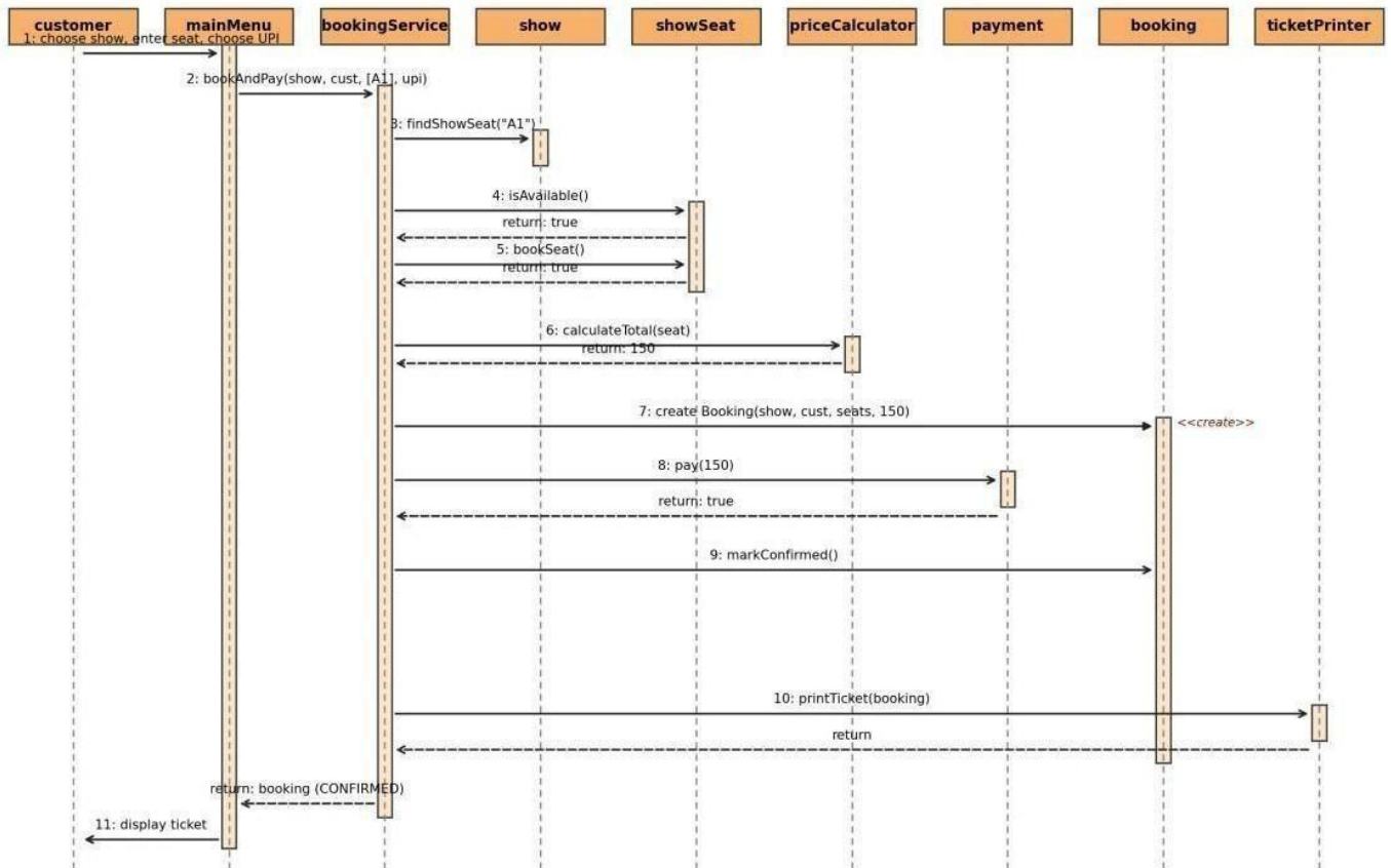
Sequence Diagram -- customer books 1 seat and pays by UPI
