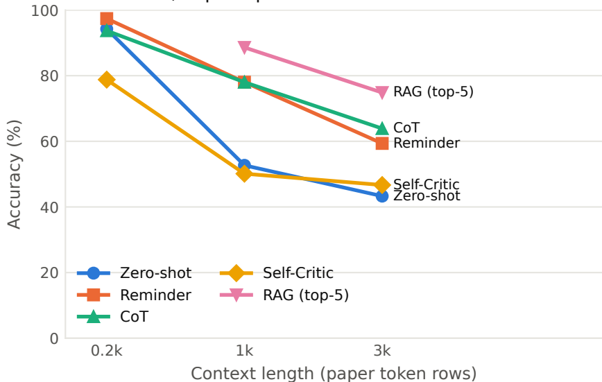
Llama-3-8B, explicit preference: all methods
