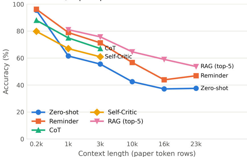
Mistral-7B, explicit preference: all methods
