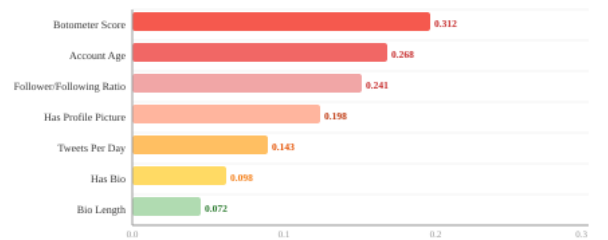
Fig. 5. Mean absolute SHAP values for the Fake class prediction across top 7 features. Higher values indicate stronger influence on the model's fake-class decision.
