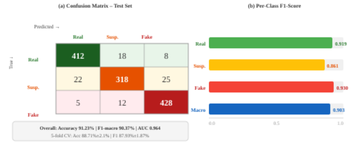
Fig. 4. (a) Confusion matrix on held-out test set ( n=1,248 ). (b) Per-class F1 scores with macro average.
