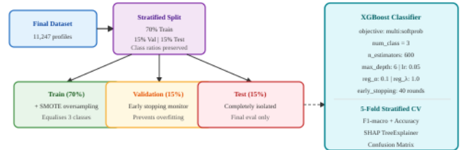
Fig. 3. XGBoost training pipeline showing stratified split, SMOTE applied only to the training fold, early stopping on the validation set, and five-fold cross-validation.
