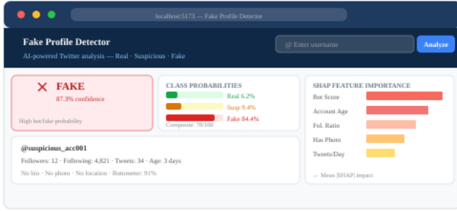
Fig. 6. React.js web interface displaying real-time classification results for a sample account. Components: LabelBadge, ScoreGauge, ProfileCard, and FeatureChart (SHAP).
