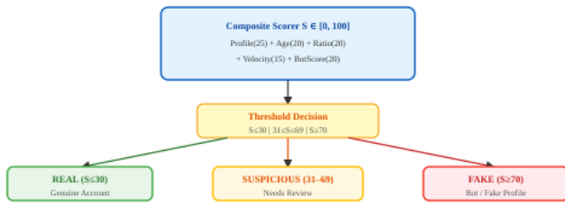
Fig. 2. Three-class labelling pipeline showing composite scoring and threshold-based label assignment.
