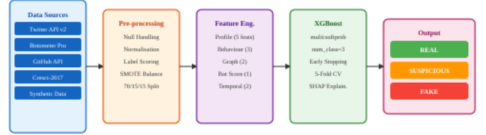
Fig. 1. End-to-end system architecture of the proposed detection framework showing data sources, preprocessing, feature engineering, XGBoost classifier, and three-class output.
