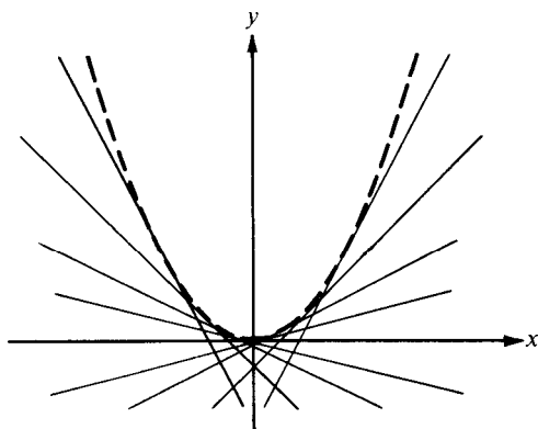
FIGURE 8.9 Integral curves of the differential equation y = x \frac{dy}{dx} - \frac{1}{4} \left( \frac{dy}{dx} \right)^2 .
