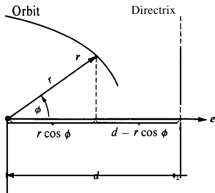
FIGURE 14.21. The ratio r/(d - r \cos \phi) is the eccentricity e = \|\mathbf{e}\| .
