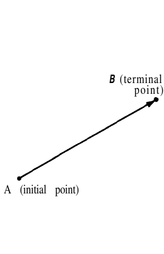
FIGURE 12.1 The geometric vector \vec{AB} from A to B .
