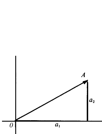
FIGURE 12.7 In V_2 , the length of A is \sqrt{a_1^2 + a_2^2} .
