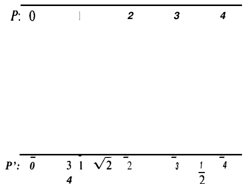
FIGURE 1.20 A partition P of [0, 4] and a refinement P' .
