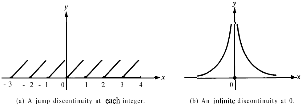
FIGURE 3.1 Illustrating two kinds of discontinuities.
