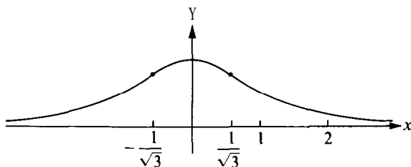
FIGURE 4.14 Graph of f(x) = 1/(x^2 + 1) .
