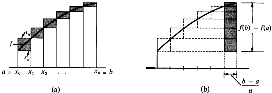
FIGURE 1.35 Proof of integrability of an increasing function.
