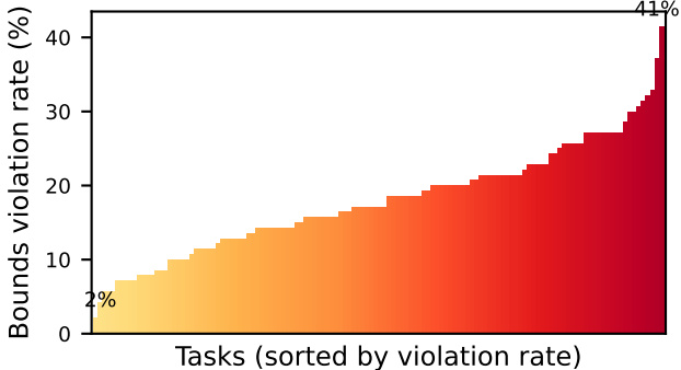
130 LIBERO Tasks: 2% to 41% spread
