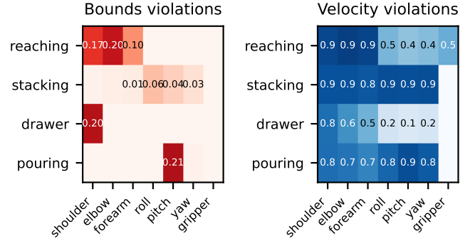
Fig. 3: Violation fingerprints across four manipulation tasks. Each task produces a distinct pattern of joint violations, enabling task identification and distribution shift detection from safety monitor logs alone.
