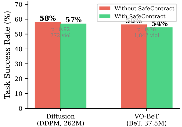
Fig. 2: Same-dataset closed-loop comparison on PushT ( n=200 per condition). VQ-BeT produces 2.4\times more violations than Diffusion Policy (1,847 vs. 772) with qualitatively different failure signatures.
