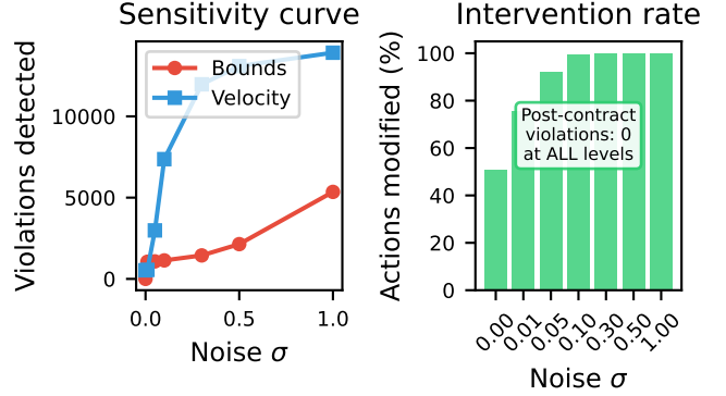
Fig. 2: Noise sensitivity calibration. Left: violations scale monotonically with noise. Right: SafeContract modifies only what is needed. Post-contract violations are zero at all noise levels.
