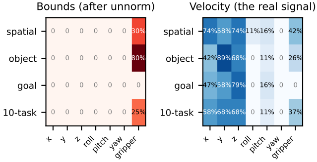
Fig. 4: Violation fingerprints after correct unnormalization. Left: bounds violations vanish (all were normalization artifacts). Right: velocity fingerprints persist and differ by task, revealing genuine behavioral patterns.
