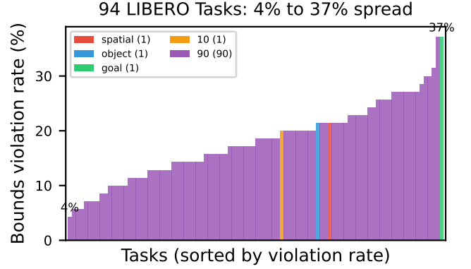
Fig. 5: Bounds violation rates across 94 LIBERO tasks (90 diverse + 4 standard suites, sorted). Rates range from 4% to 37%, with standard suite tasks (colored) distributed across the spectrum.
