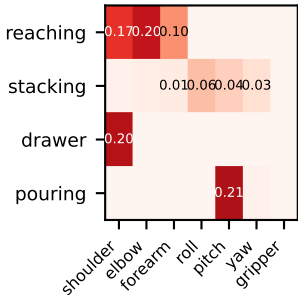
Bounds violations
