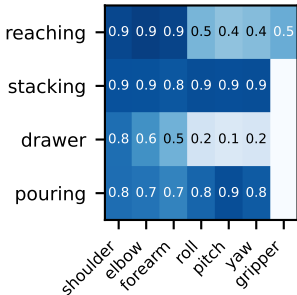
Velocity violations
