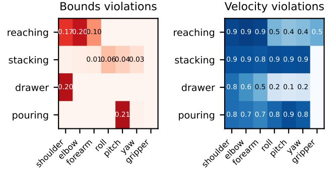
Fig. 3: Violation fingerprints across four manipulation tasks. Each task produces a distinct pattern of joint violations, enabling task identification and distribution shift detection from safety monitor logs alone.
