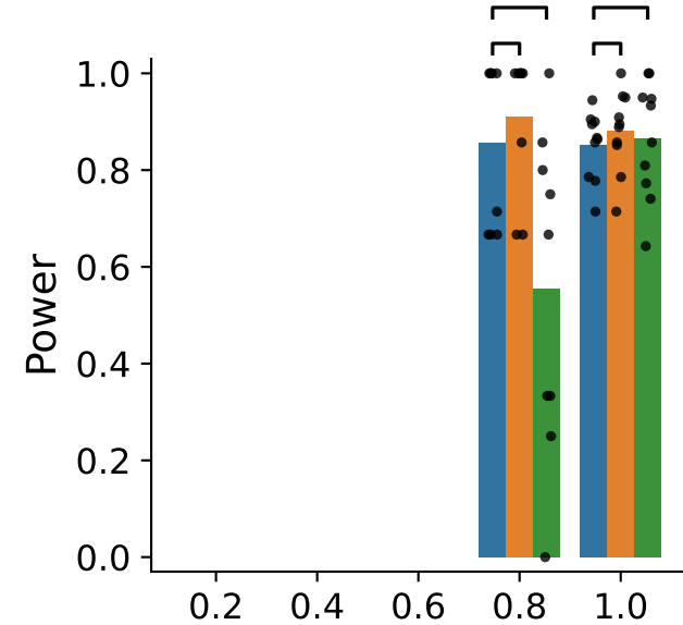
Cell type bin 1: 30-39
