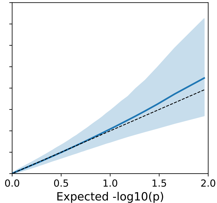
Metacell size: 75
