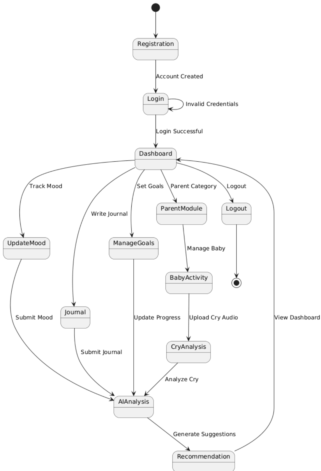
NeuroSync - State Chart Diagram
