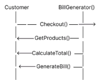
Sequence Diagram
