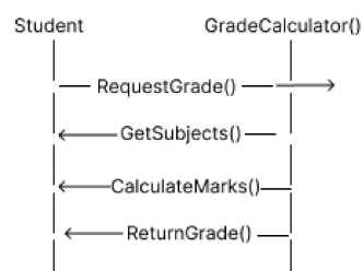
Sequence Diagram
