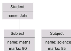
Object Diagram
