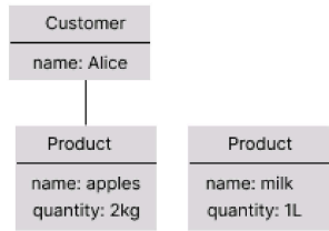
Object Diagram
