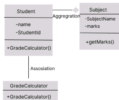
Class Diagram
