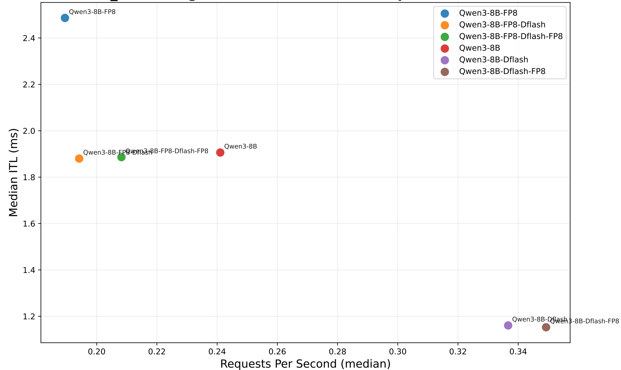
math_reasoning - Median ITL (ms) vs Requests Per Second
