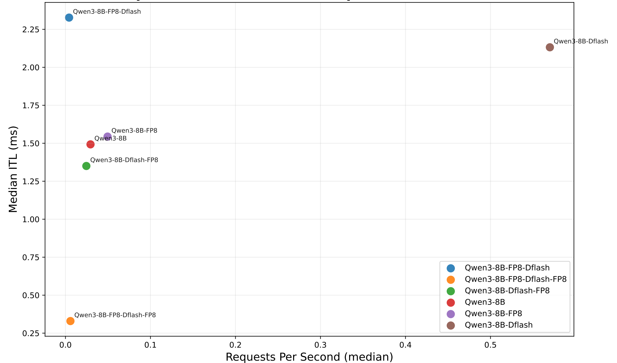
qa - Median ITL (ms) vs Requests Per Second
