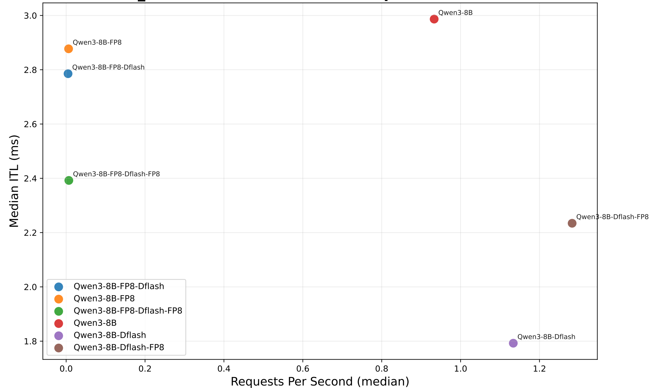
tool_call - Median ITL (ms) vs Requests Per Second
