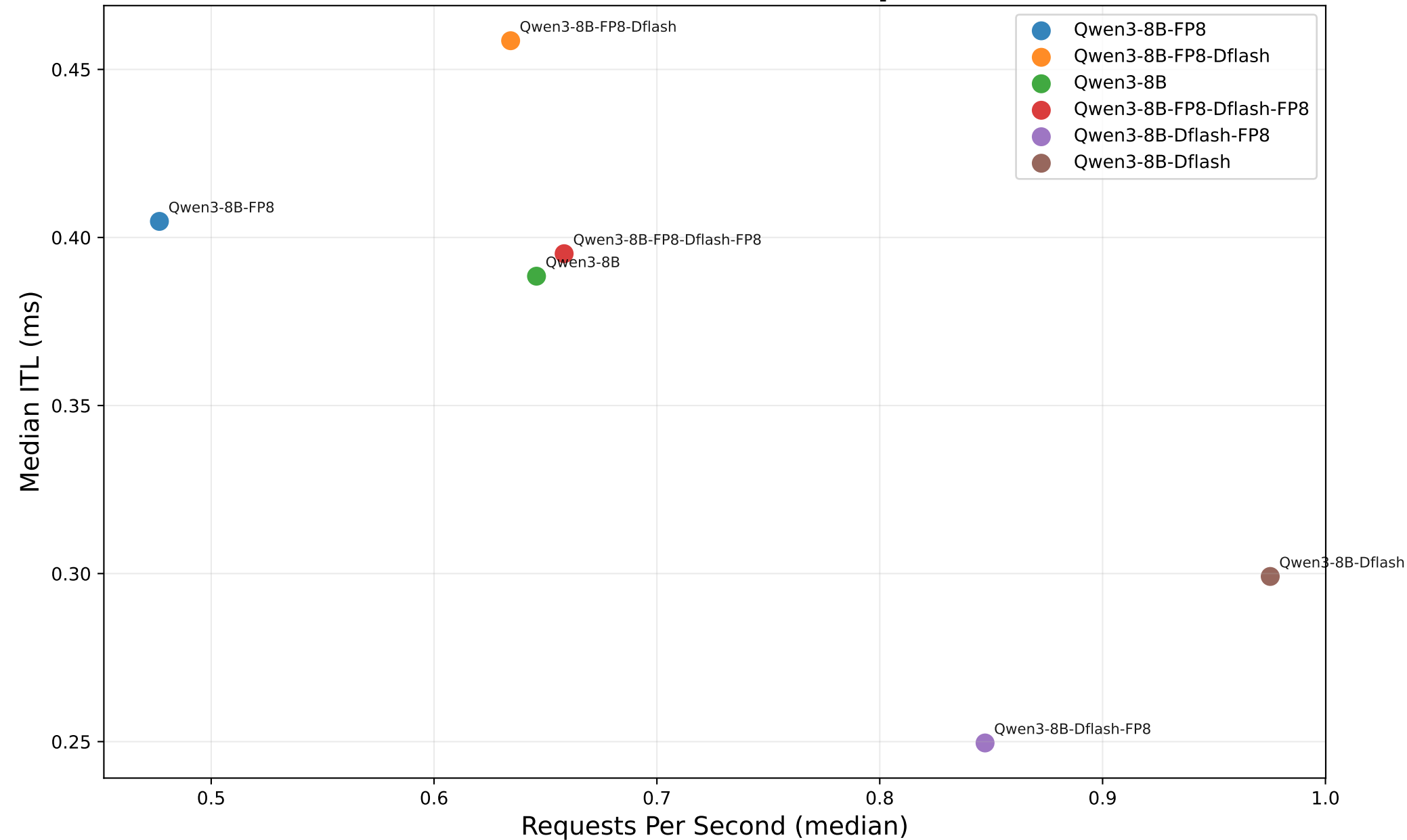
translation - Median ITL (ms) vs Requests Per Second
