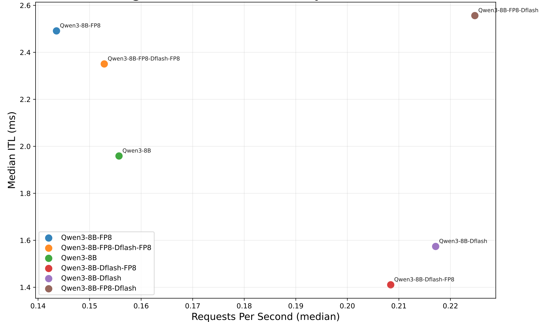
writing - Median ITL (ms) vs Requests Per Second
