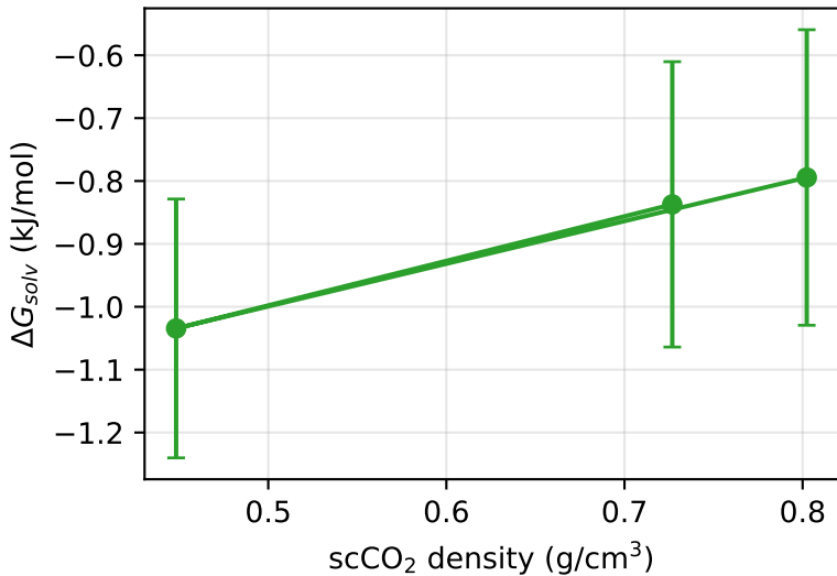
CH 4 solvation free energy vs scCO 2 density
