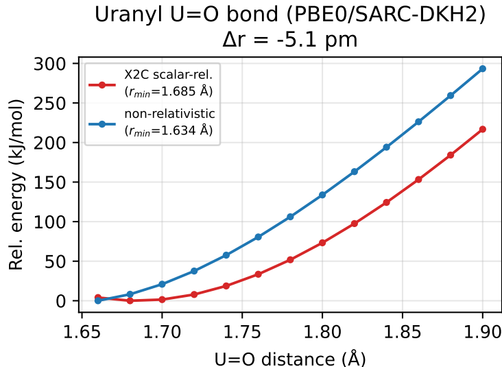
Figure 1: Uranyl U=O potential energy curve (PBE0/SARC-DKH2) with and without the scalar-X2C Hamiltonian (same basis). The relativistic reference geometry is r(\text{U=O}) = 1.685 \text{ Å} .
